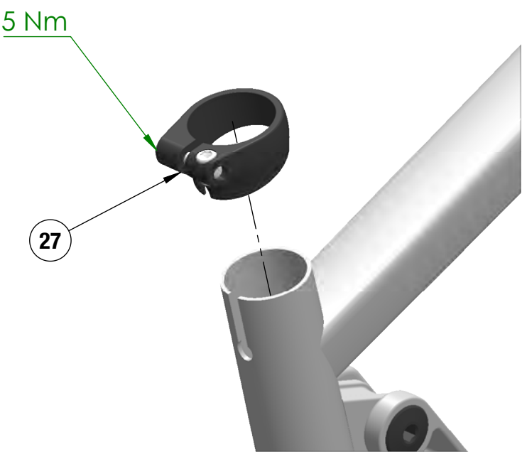
SEATPOST CLAMP
