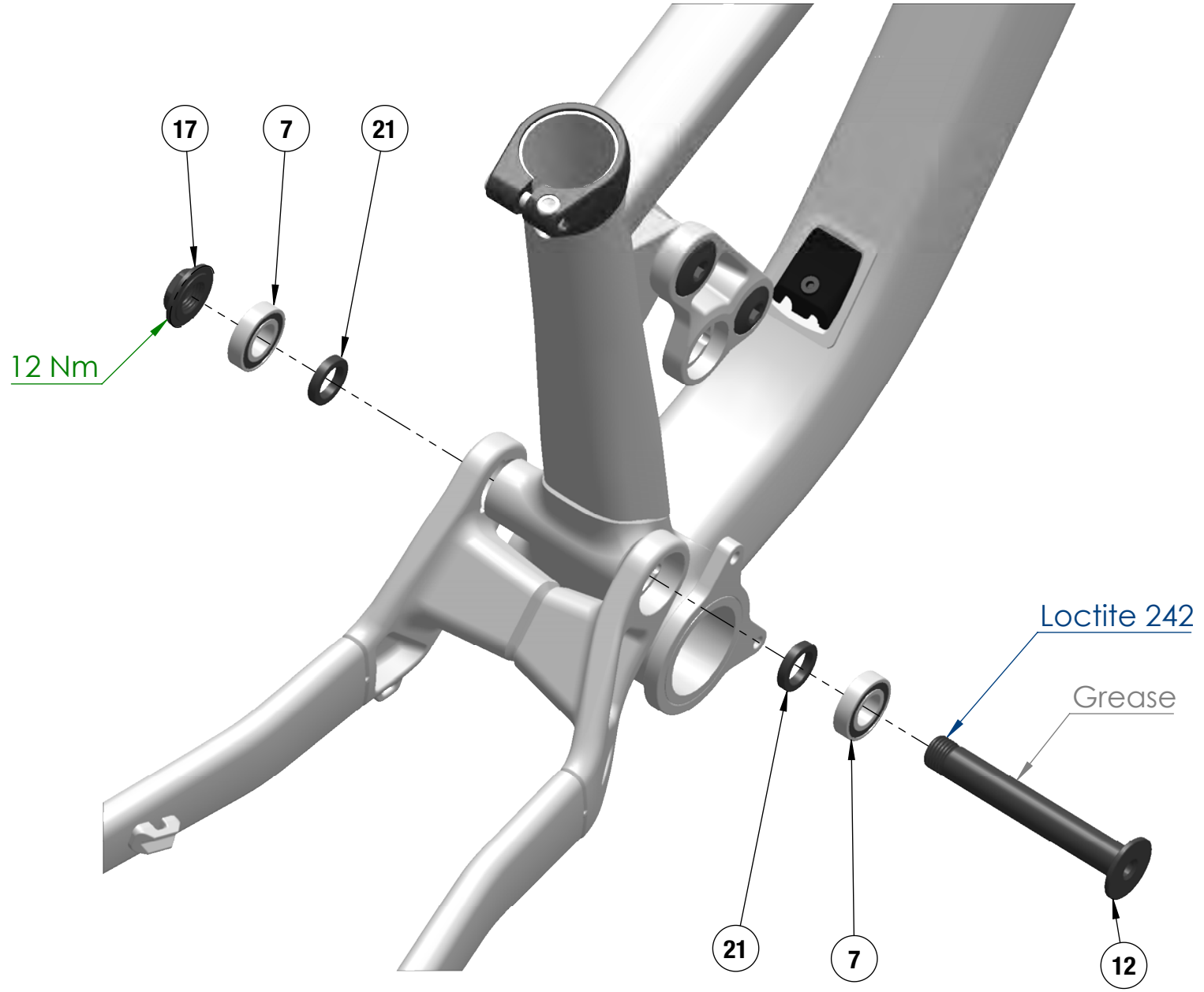
MAIN PIVOT
