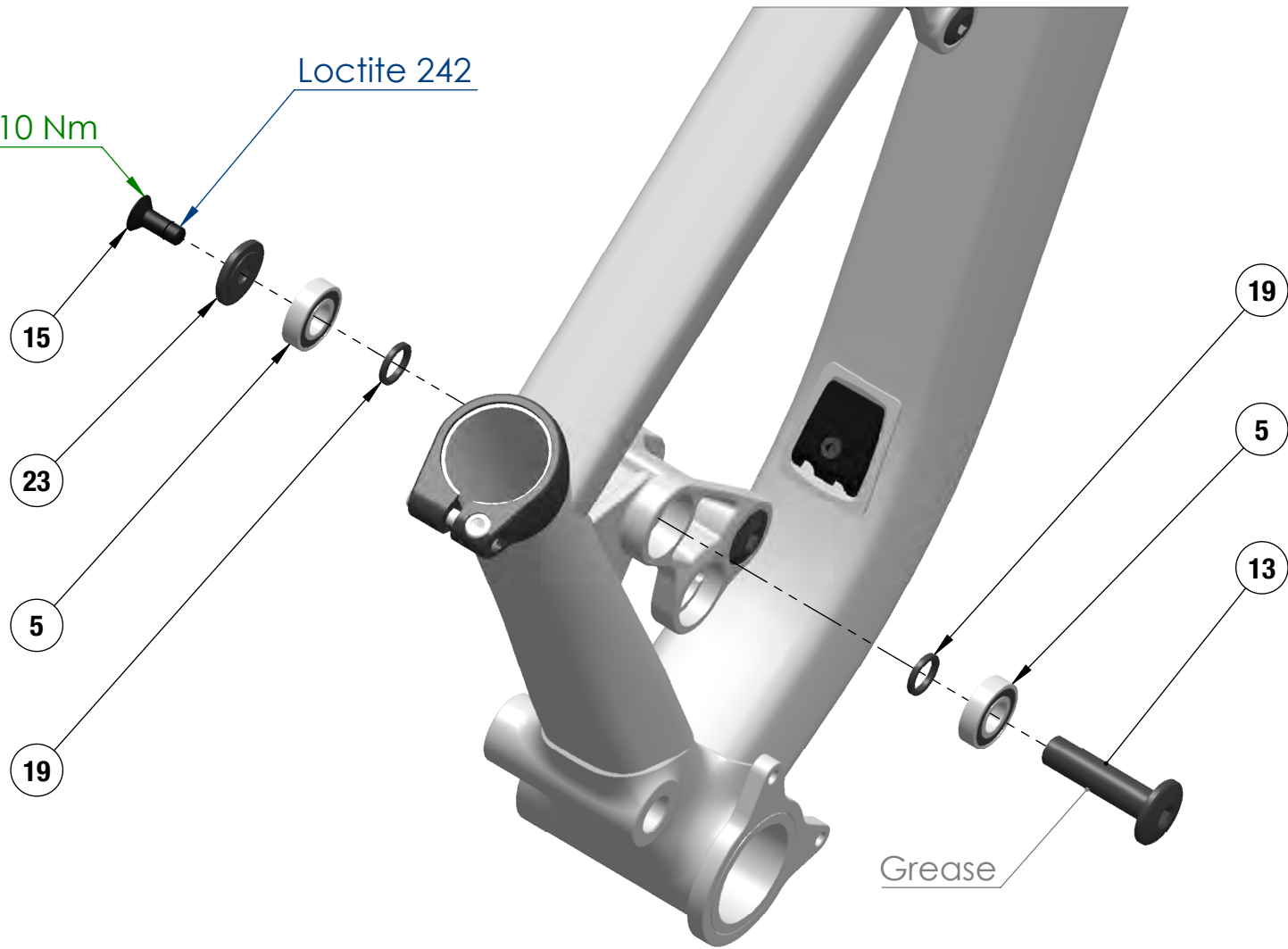
LINKARM FIXED PIVOT
