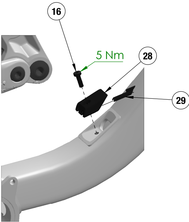
DOWNTUBE CABLE EXIT
