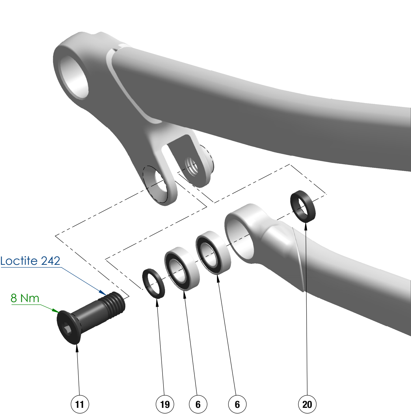
HORST PIVOT MIRRORED ARRANGEMENT ON NON-DRIVE SIDE
