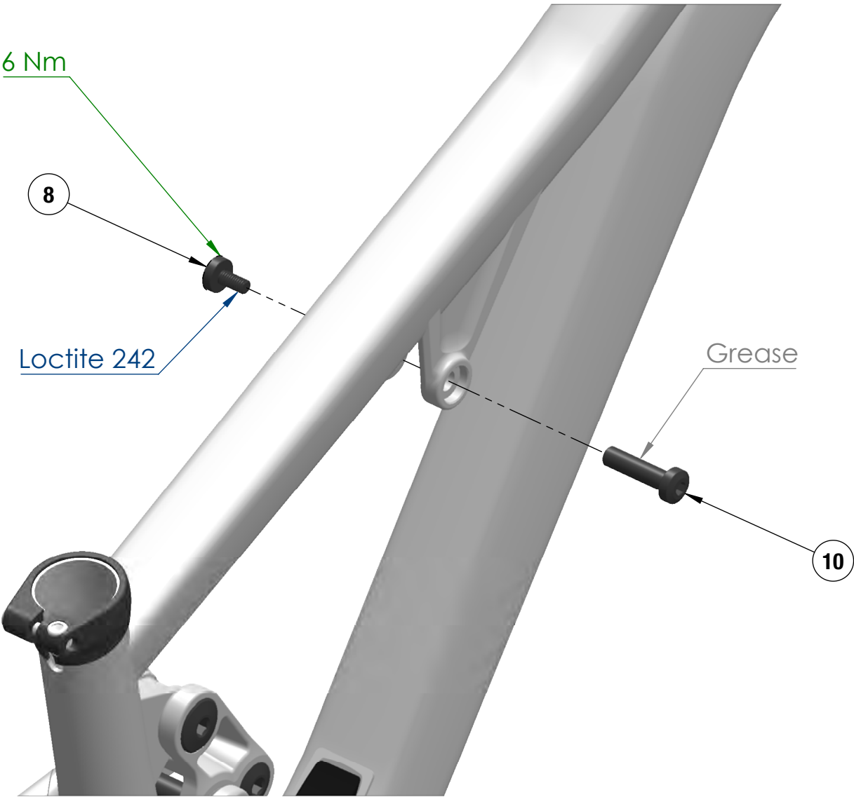
SHOCK FIXED PIVOT
