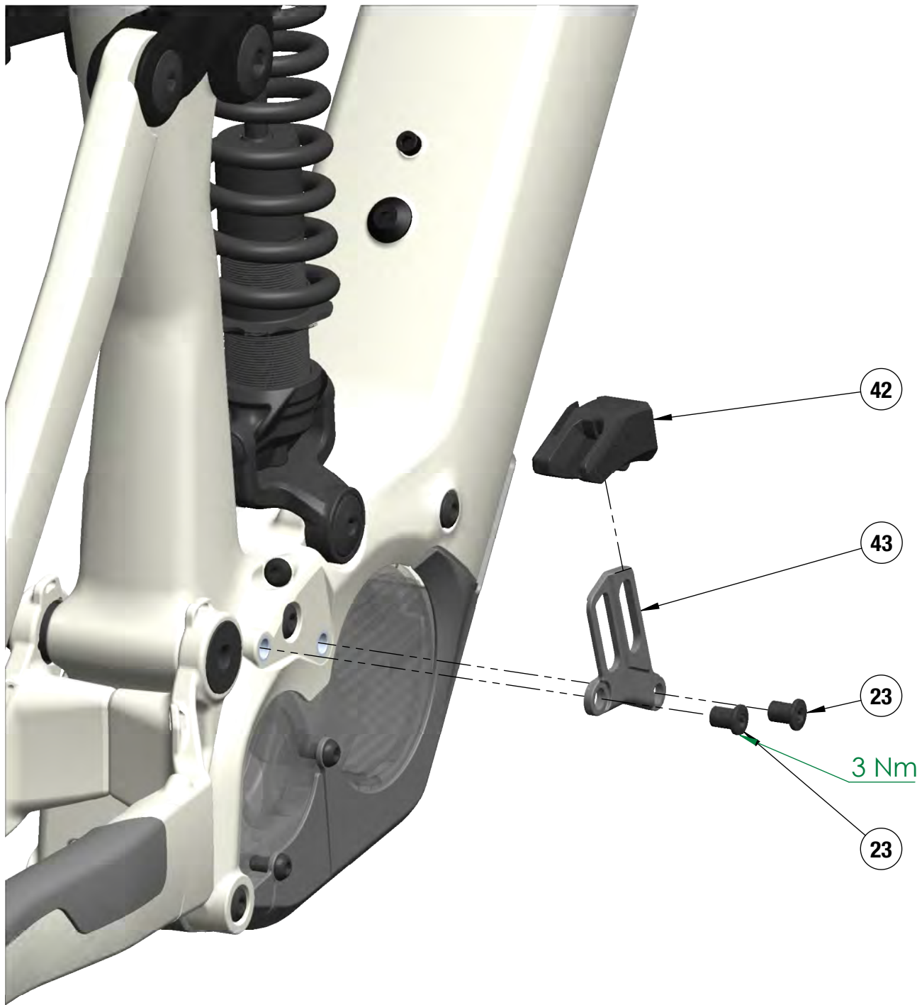
CHAINGUIDE INSTALL
