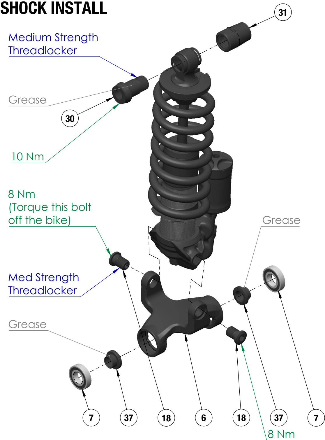
SHOCK HARDWARE
