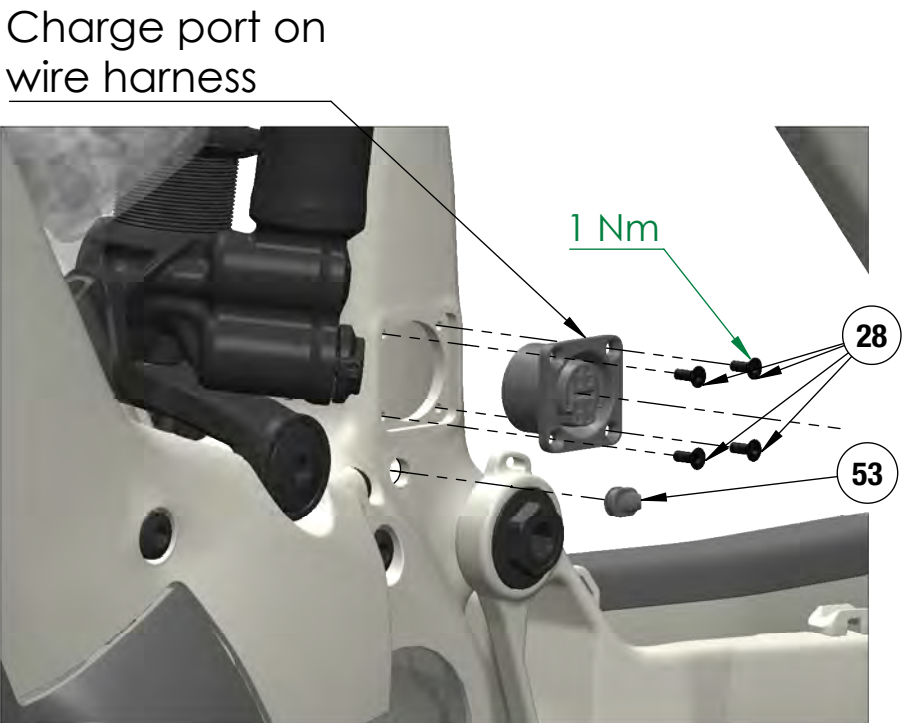
CHARGE PORT INSTALL
