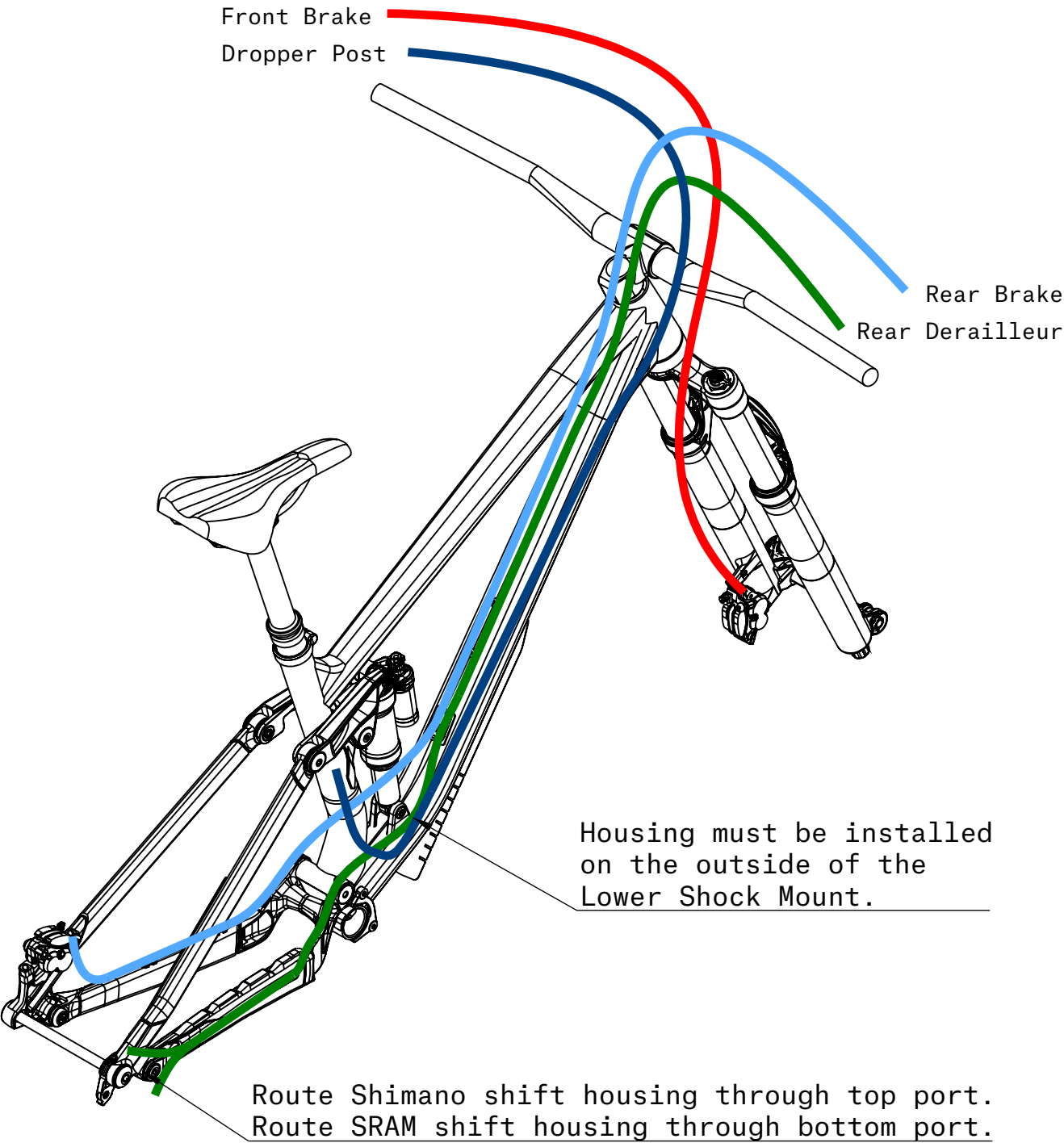
STANDARD LAYOUT - ISOMETRIC VIEW
