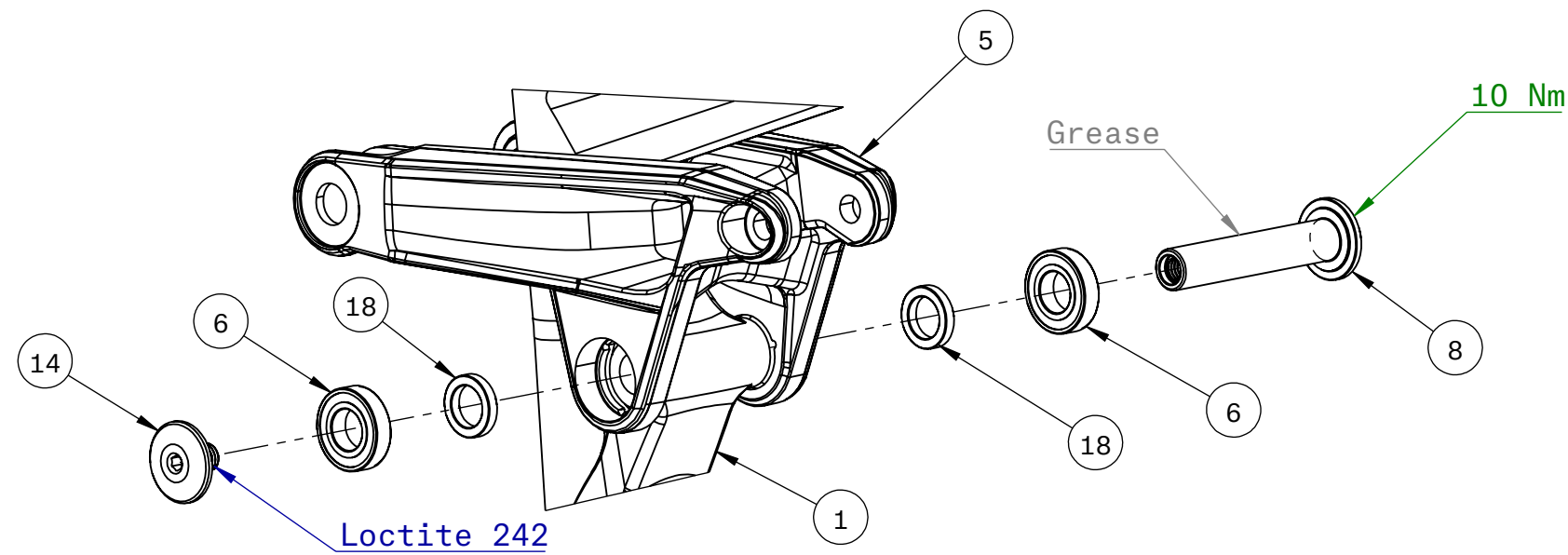
LINKARM TO FRONT TRIANGLE PIVOT
