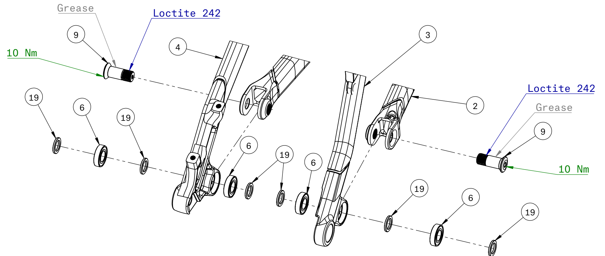
CHAIN STAY TO SEAT STAY PIVOT
