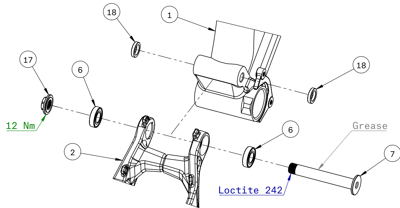
CHAIN STAY TO FRONT TRIANGLE PIVOT
