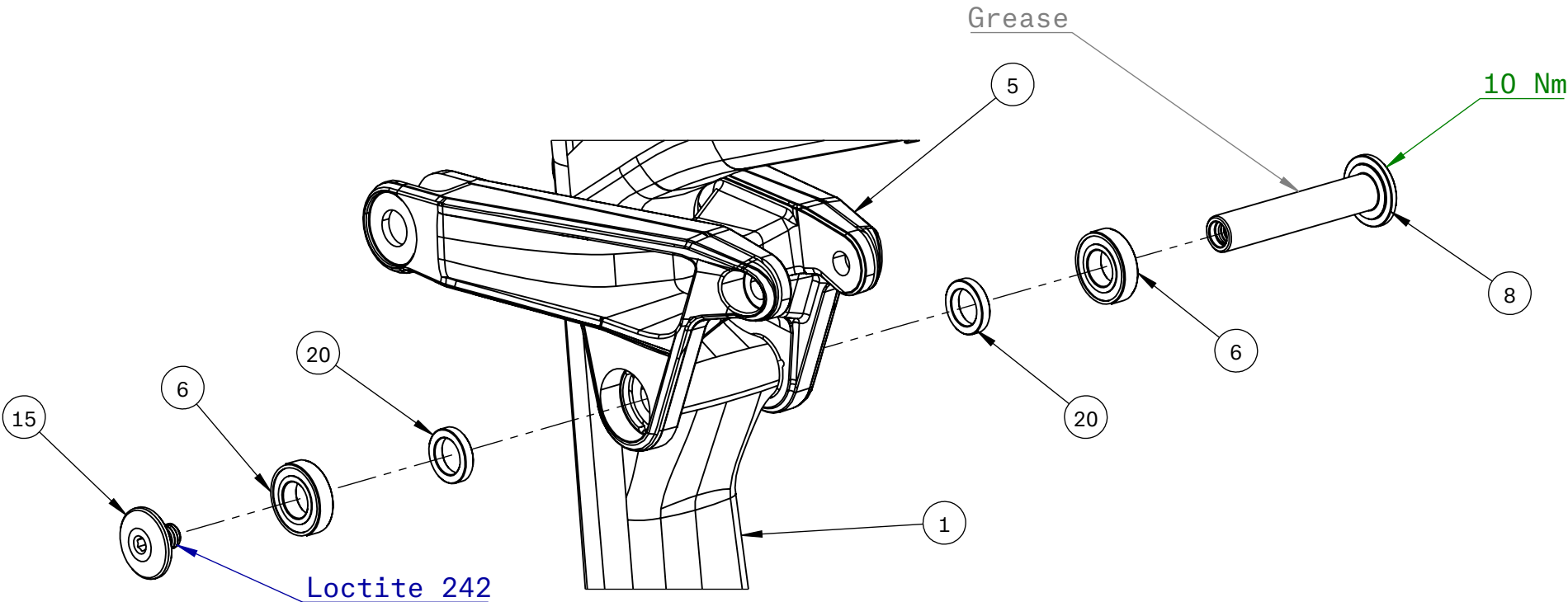
LINKARM TO FRONT TRIANGLE PIVOT
