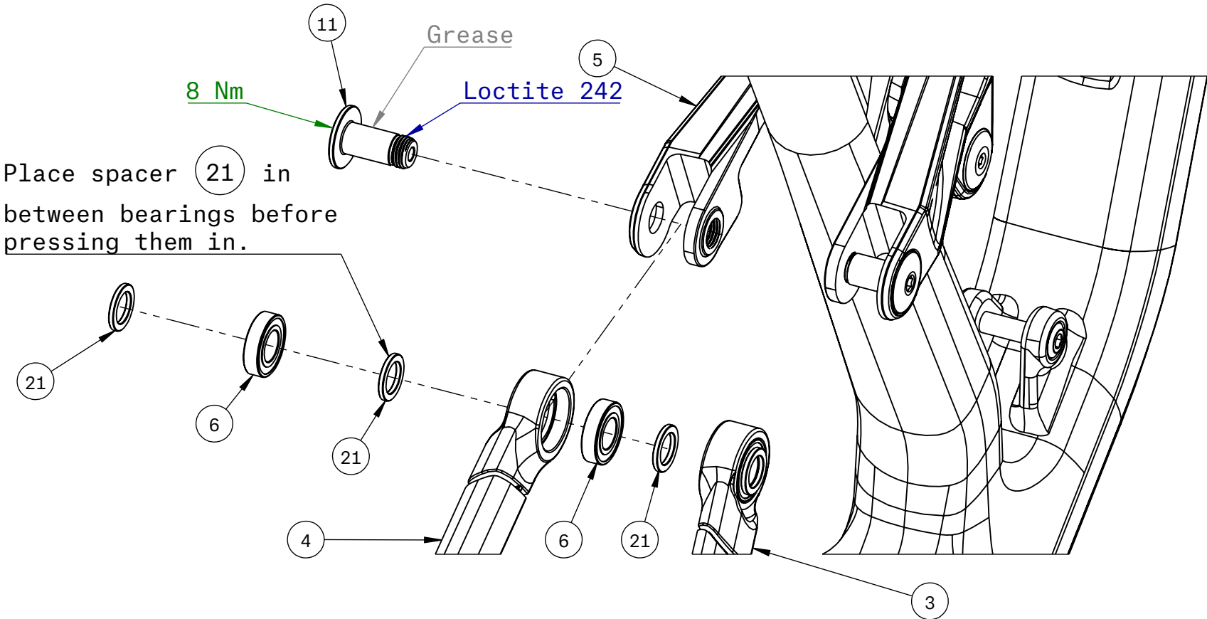
LINKARM TO SEAT STAY PIVOT MIRRORED ARRANGEMENT ON RIGHT SEAT STAY
