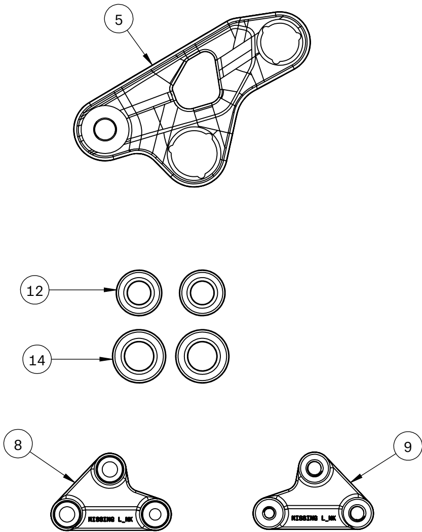
29" rear wheel kit, Optic Carbon
