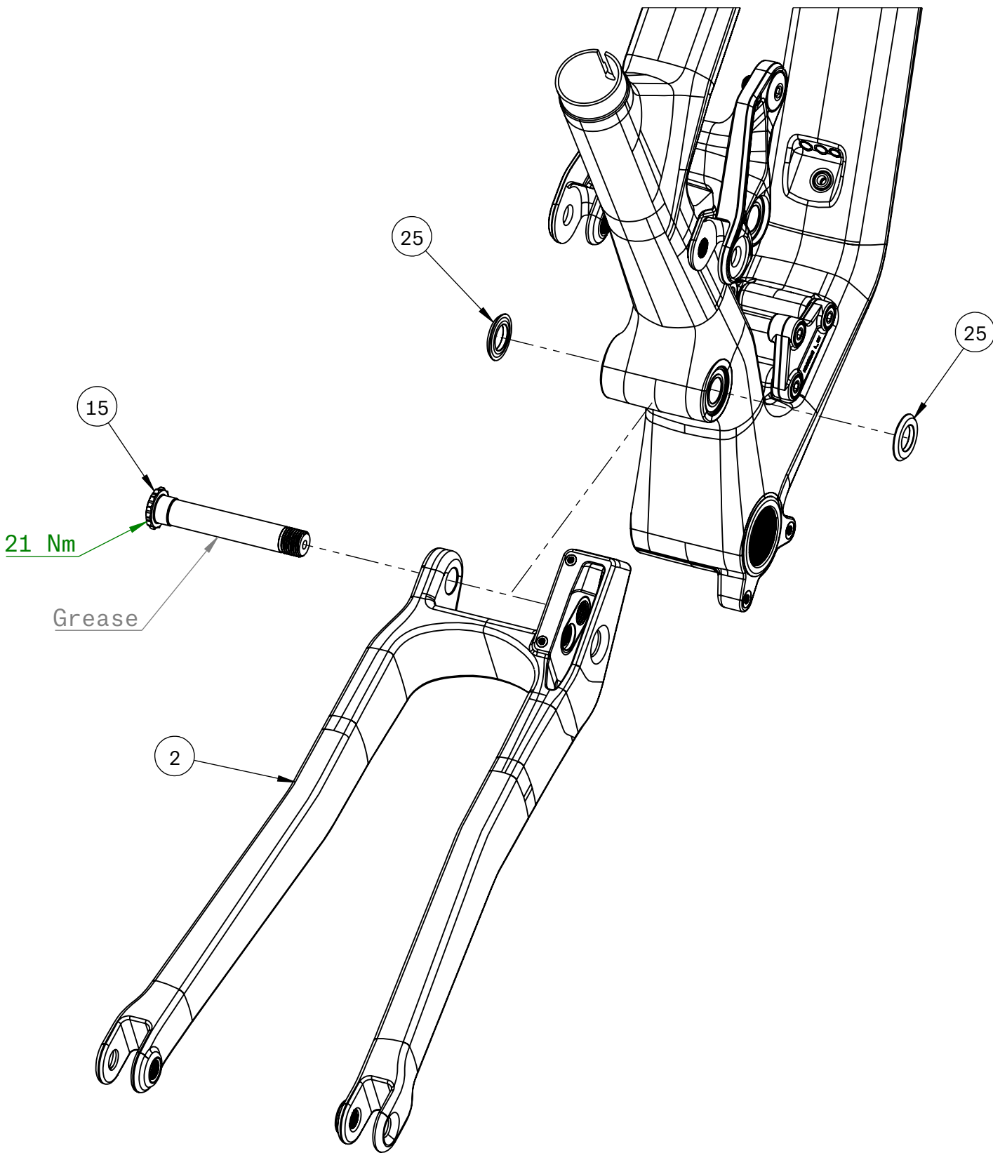
Front Triangle to Chain Stay
