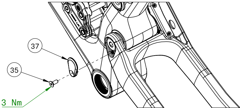
Main Pivot Shaft Retainer
