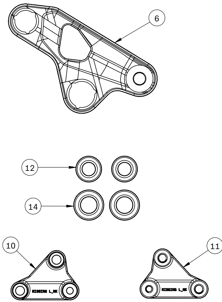
27.5" rear wheel kit, Optic Carbon
