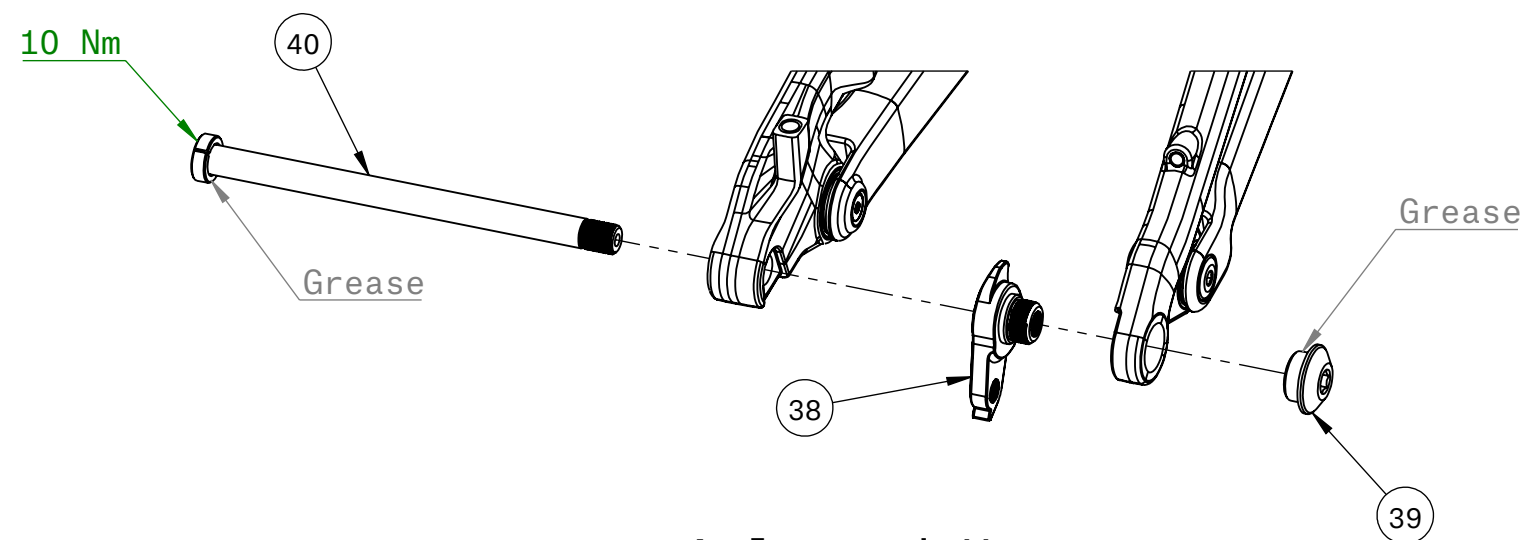
Axle and Hanger
