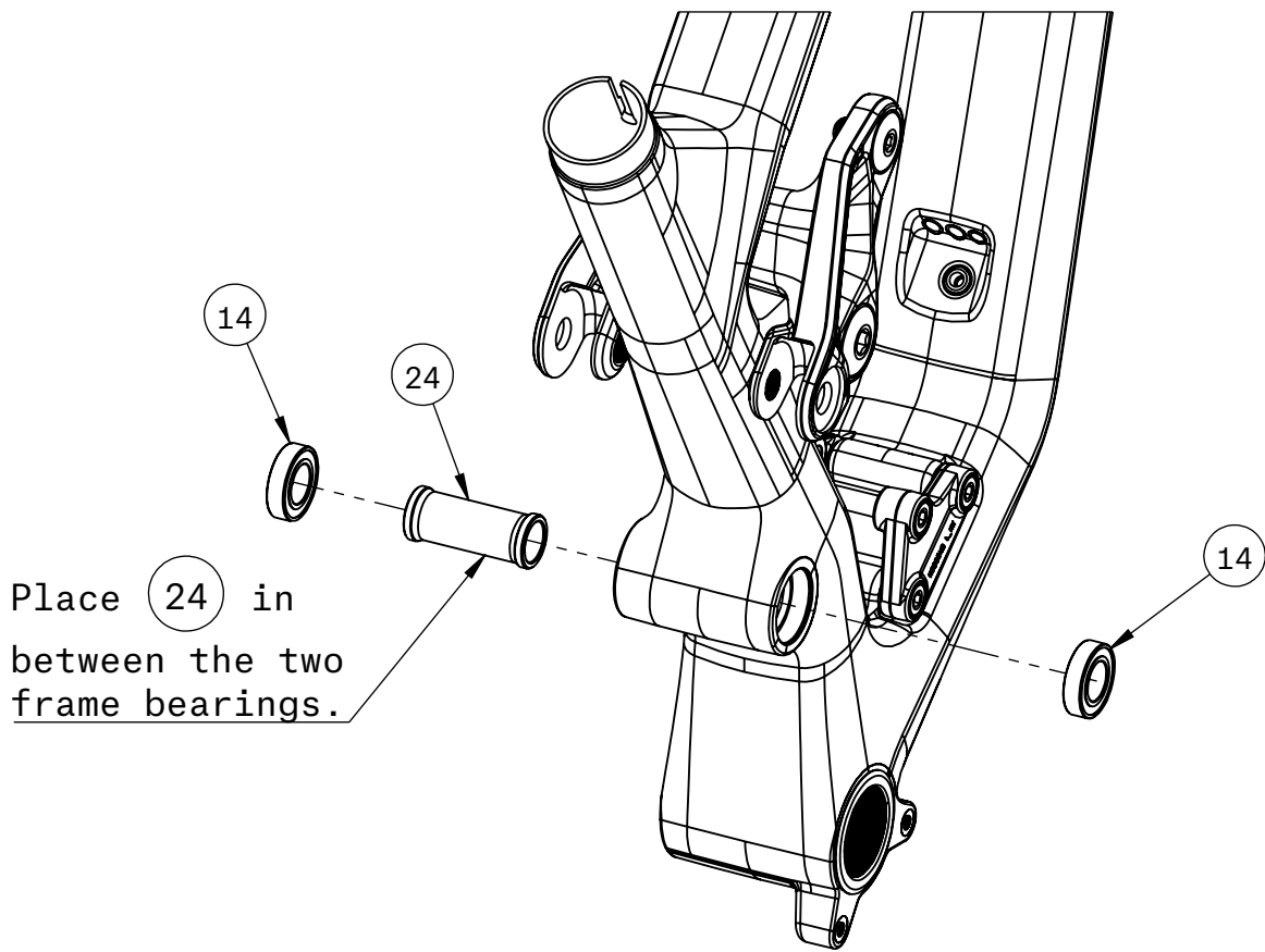
Front Triangle Bearings
