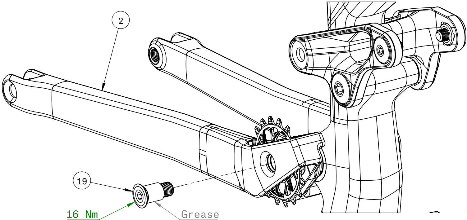
Idler to Chain Stay
