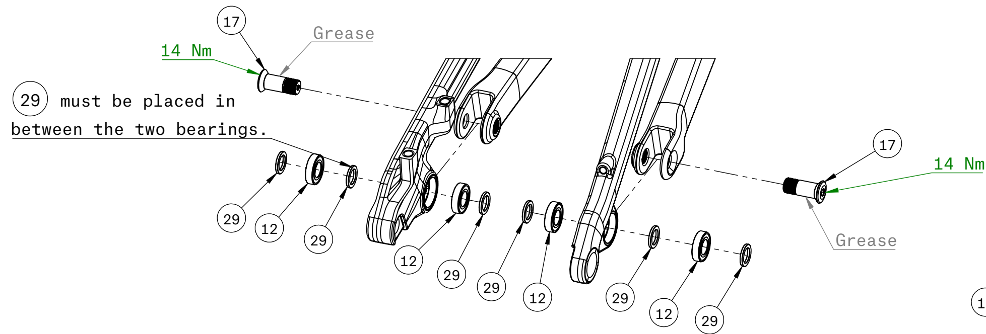
Chain Stay to Seat Stays
