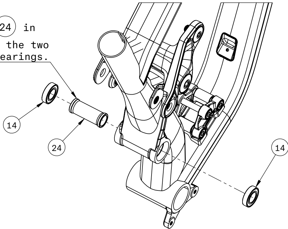
Front Triangle Bearings
