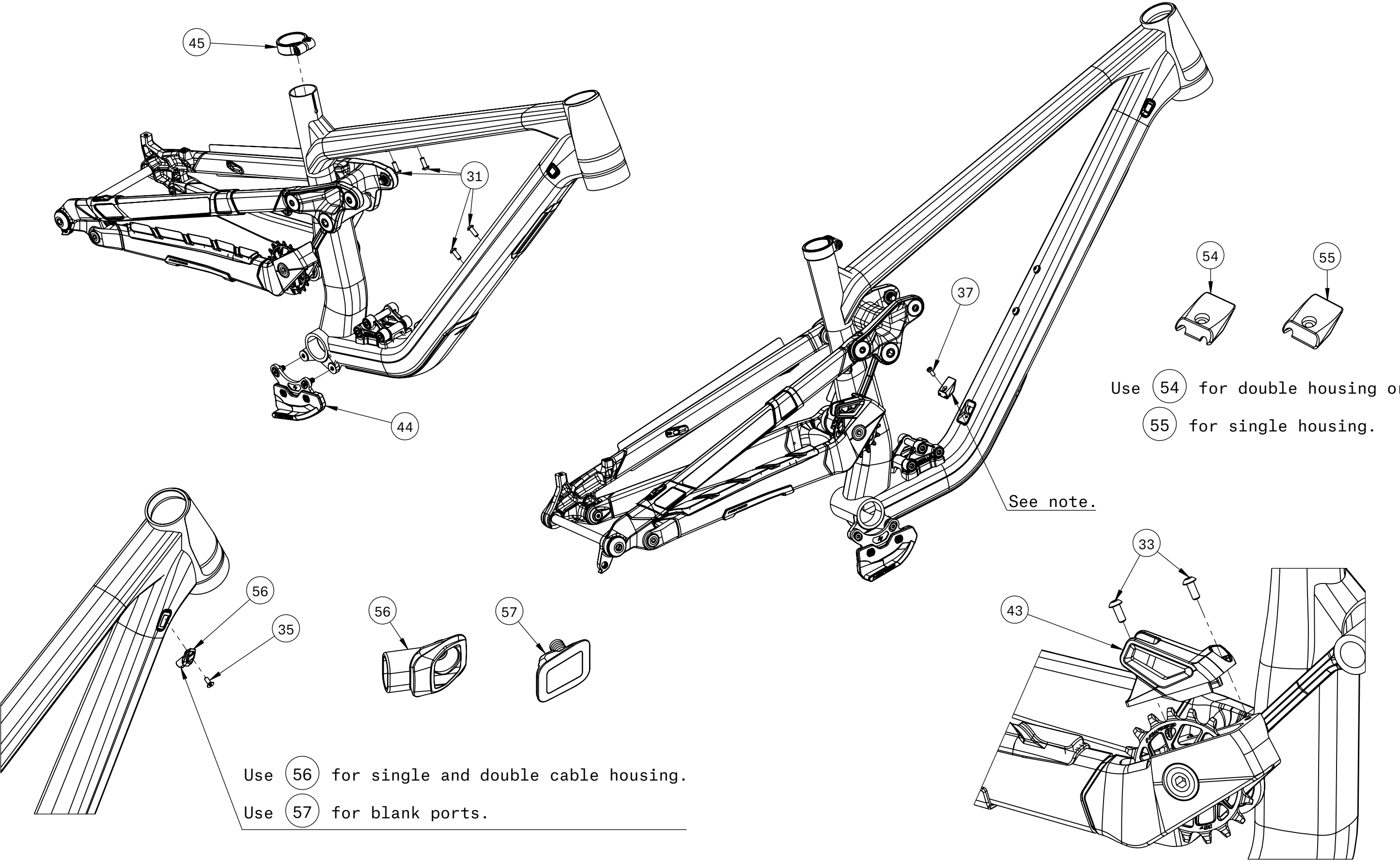
Head Tube Cable Port
