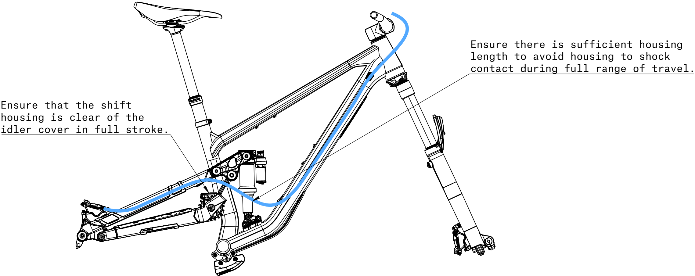
Route brake and shift housing as shown.
