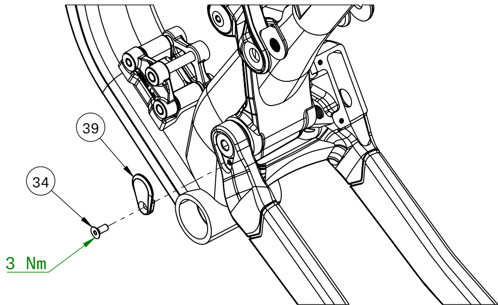
Main Pivot Shaft Retainer
