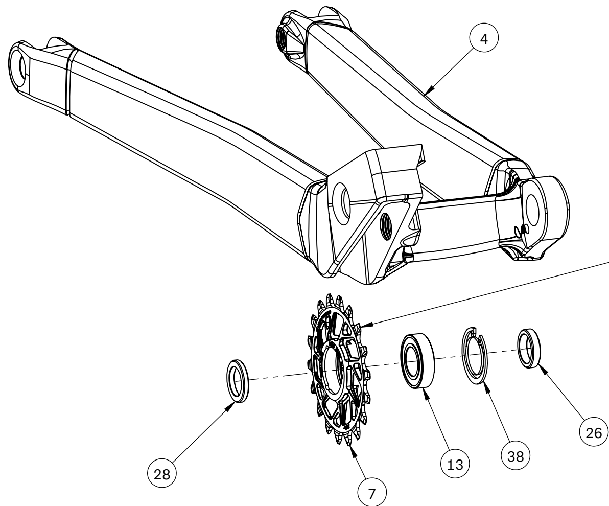
Idler Hardware Arrangement
