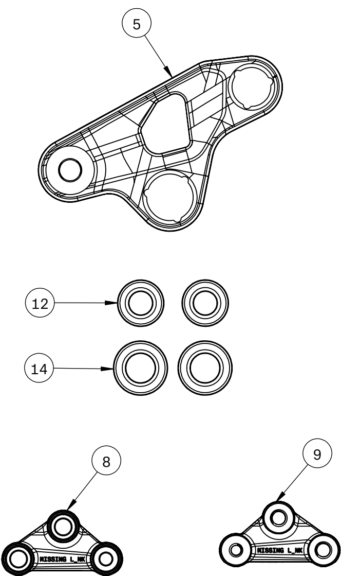
29" rear wheel kit, Sight Aluminum
