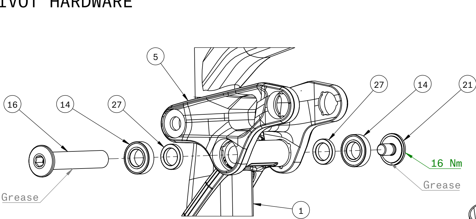
Linkarm to Front Triangle
