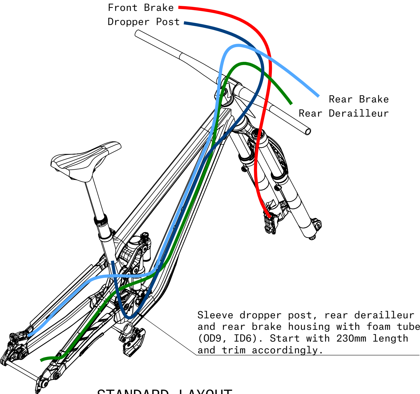
STANDARD LAYOUT ISOMETRIC VIEW
