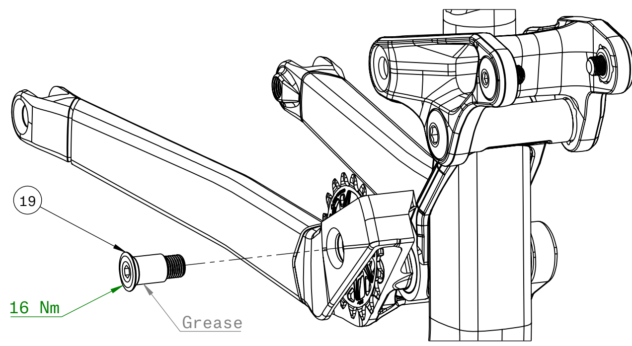
Idler to Chain Stay
