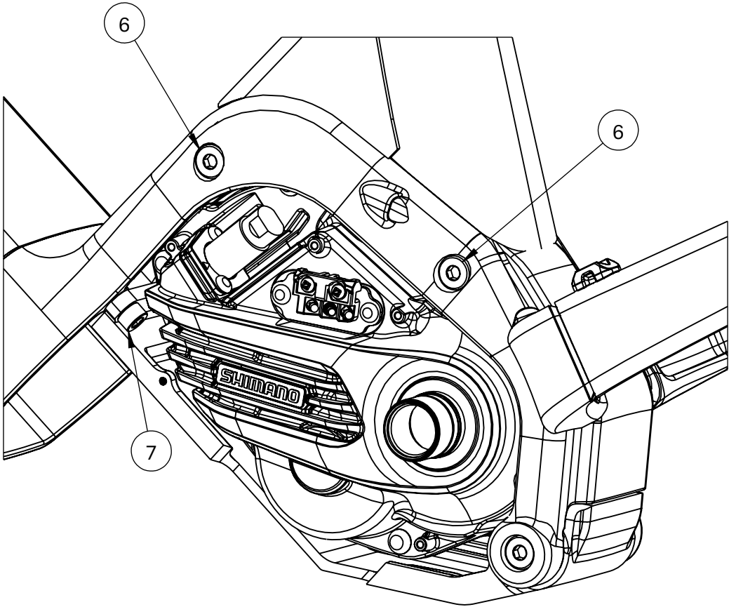
SUBFRAME NON-DRIVE SIDE VIEW
