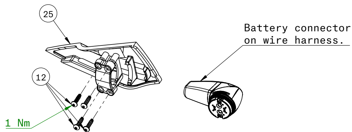
CHARGE PORT DOOR ASSEMBLY
