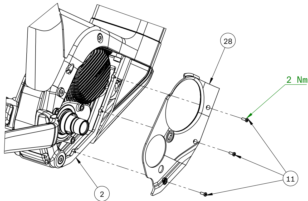
RIGHT DRIVE UNIT COVER
