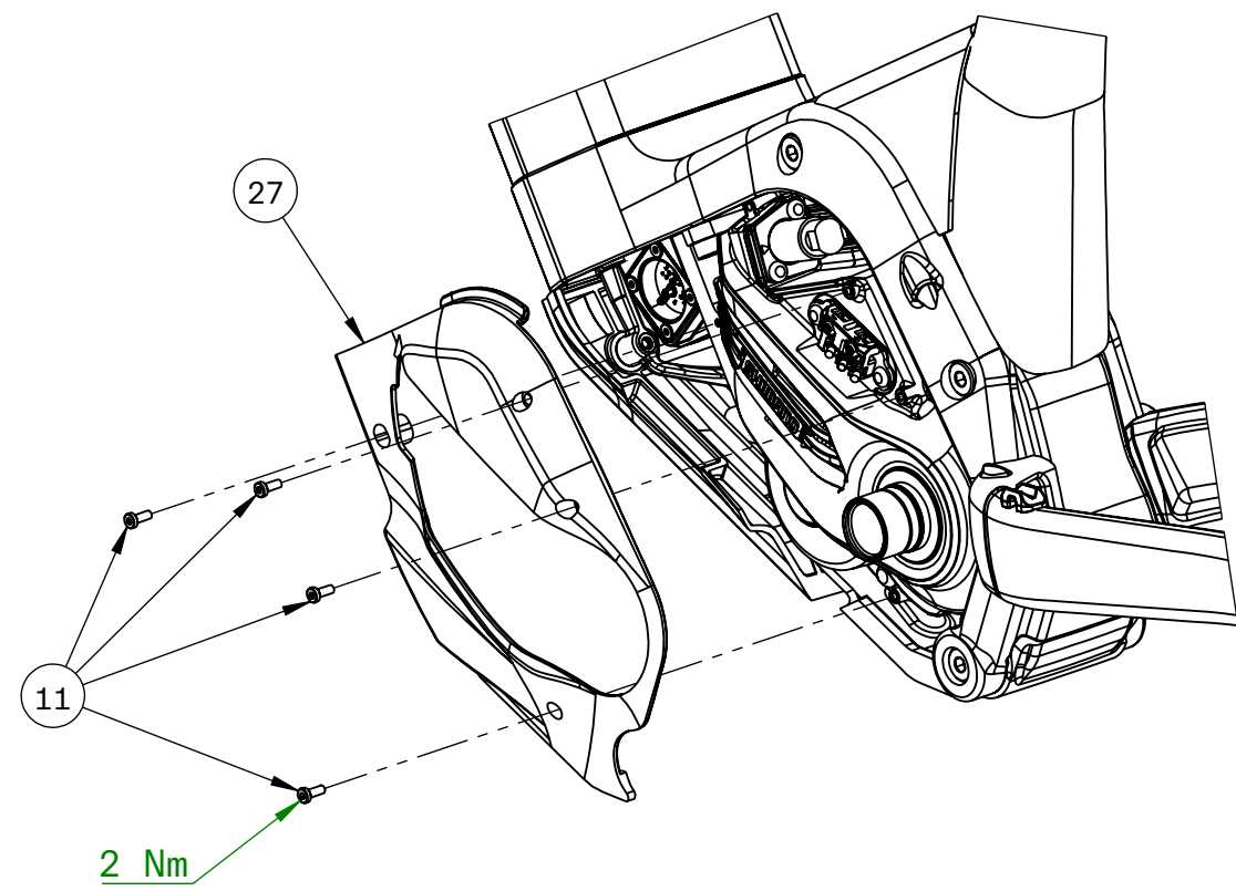
LEFT DRIVE UNIT COVER
