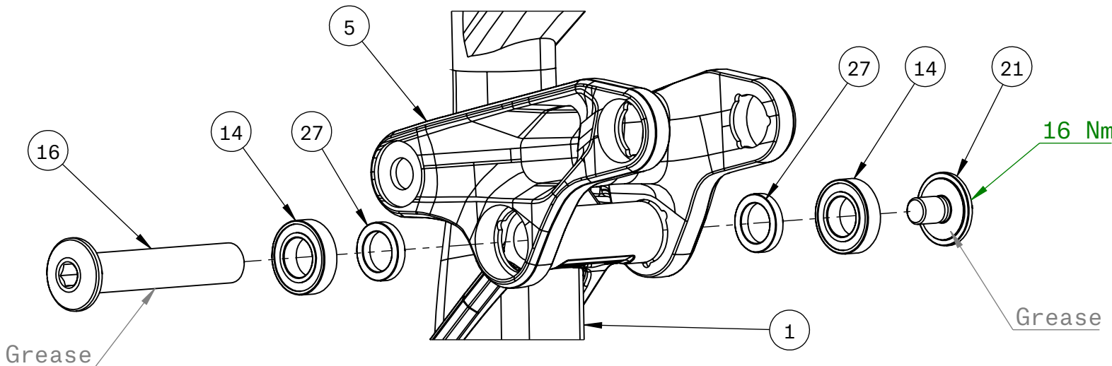
Linkarm to Front Triangle
