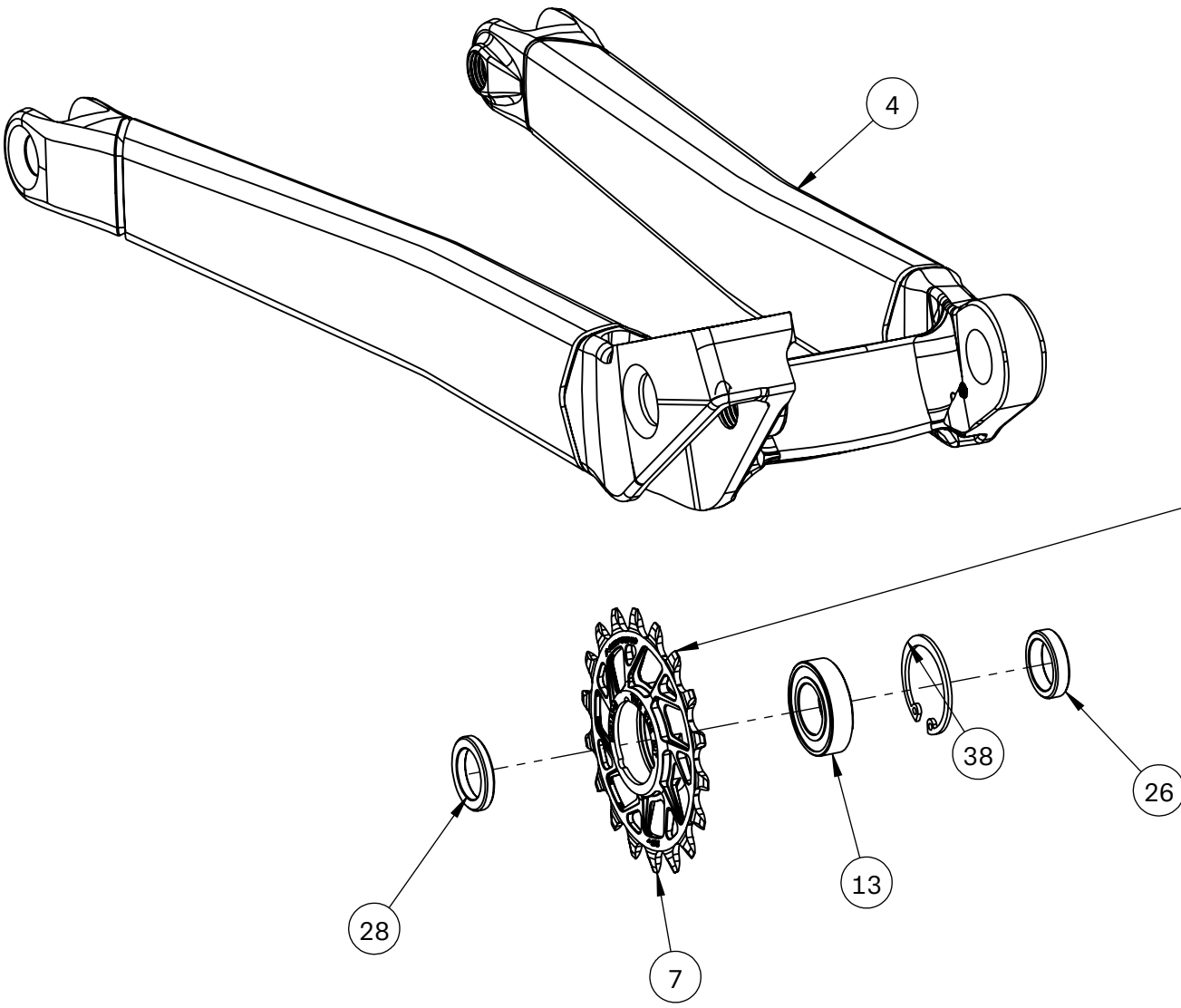
Idler Hardware Arrangement
