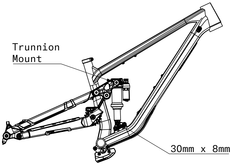
Shock Orientation
