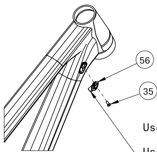
Head Tube Cable Ports
