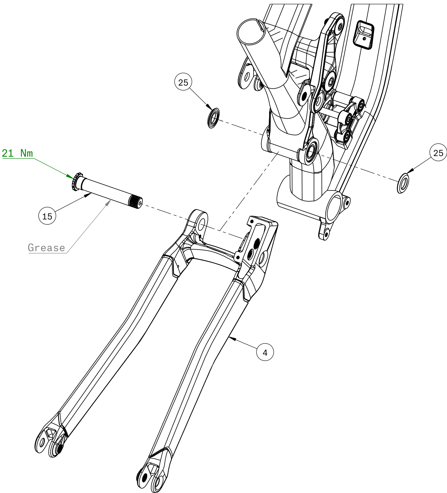
Front Triangle to Chain Stay
