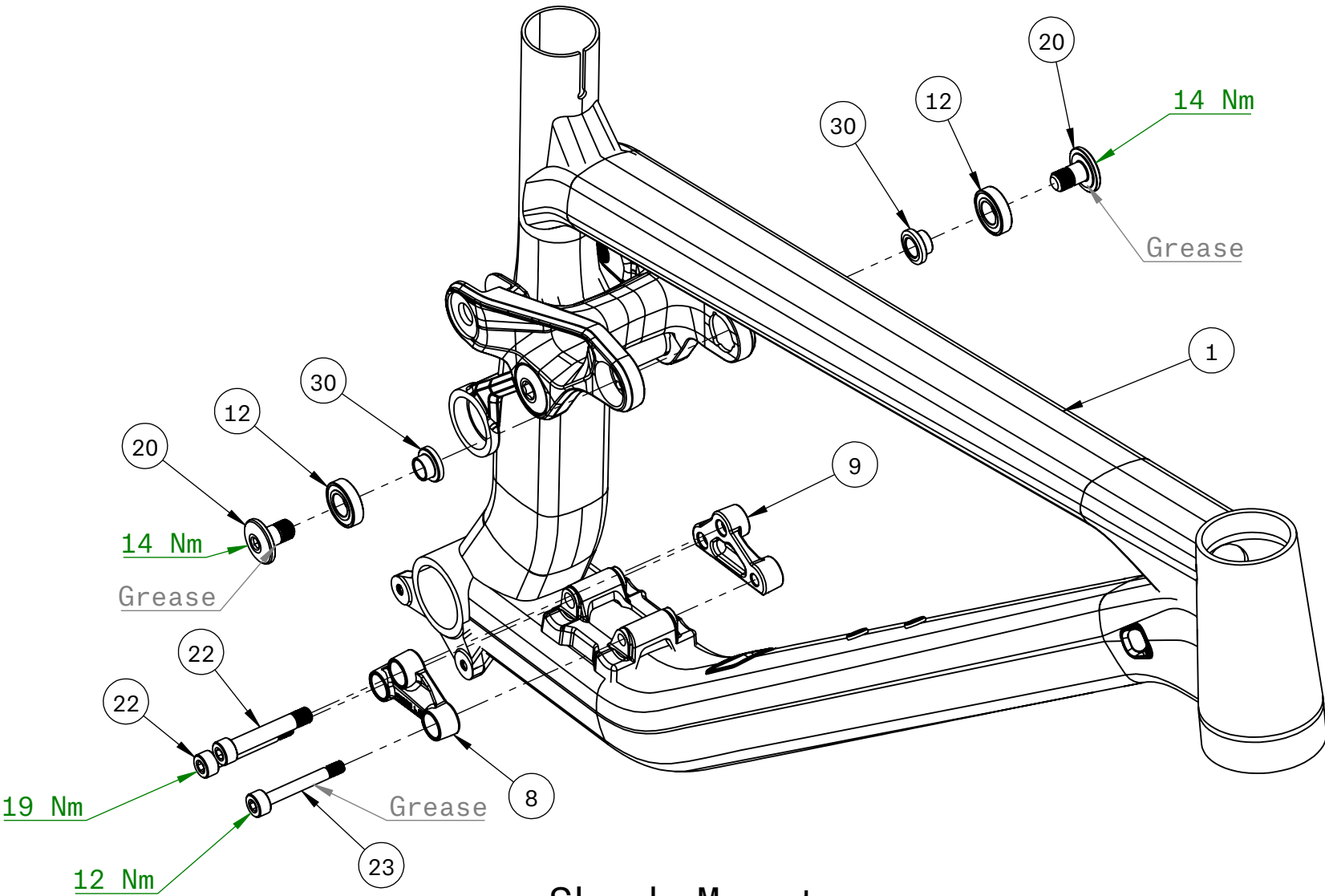
Shock Mounts
