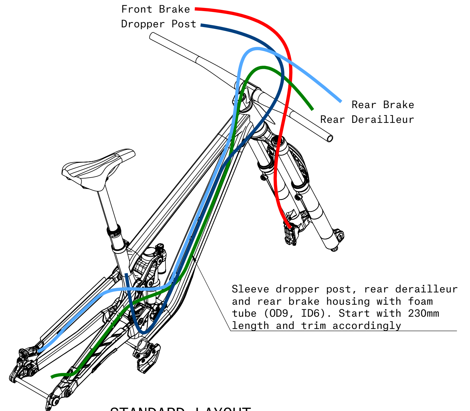
STANDARD LAYOUT ISOMETRIC VIEW
