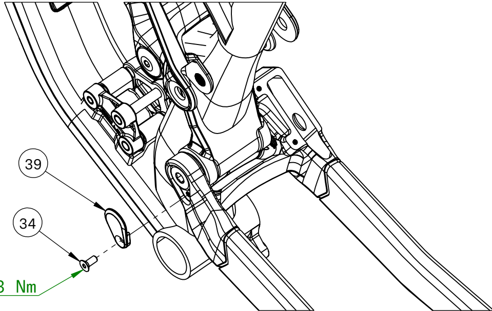
Main Pivot Shaft Retainer
