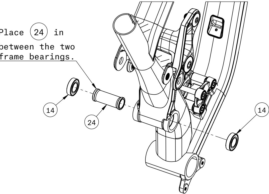
Front Triangle Bearings
