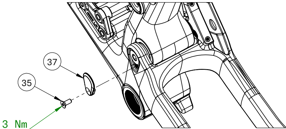
Main Pivot Shaft Retainer
