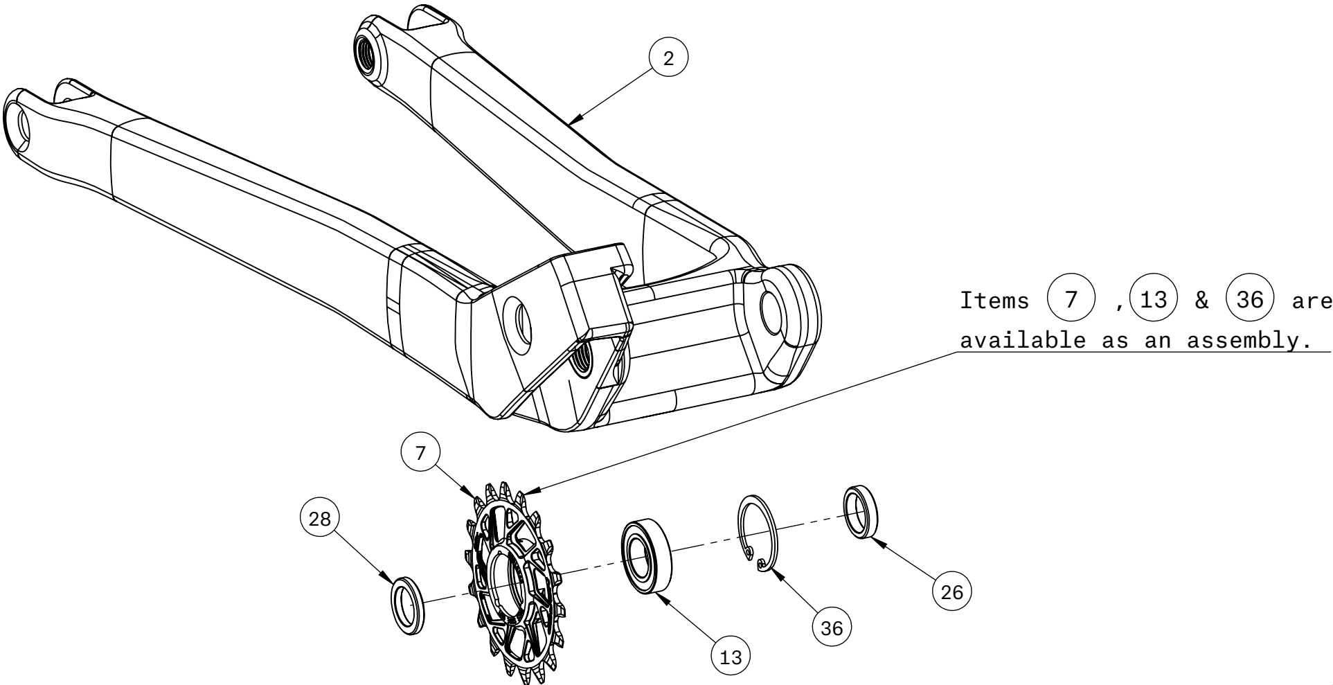
Idler Hardware Arrangement
