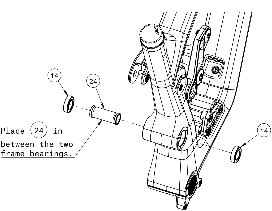
Front Triangle Bearings
