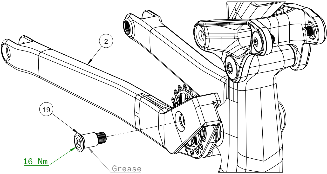
Idler to Chain Stay
