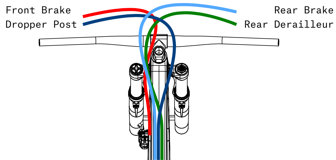
STANDARD LAYOUT
