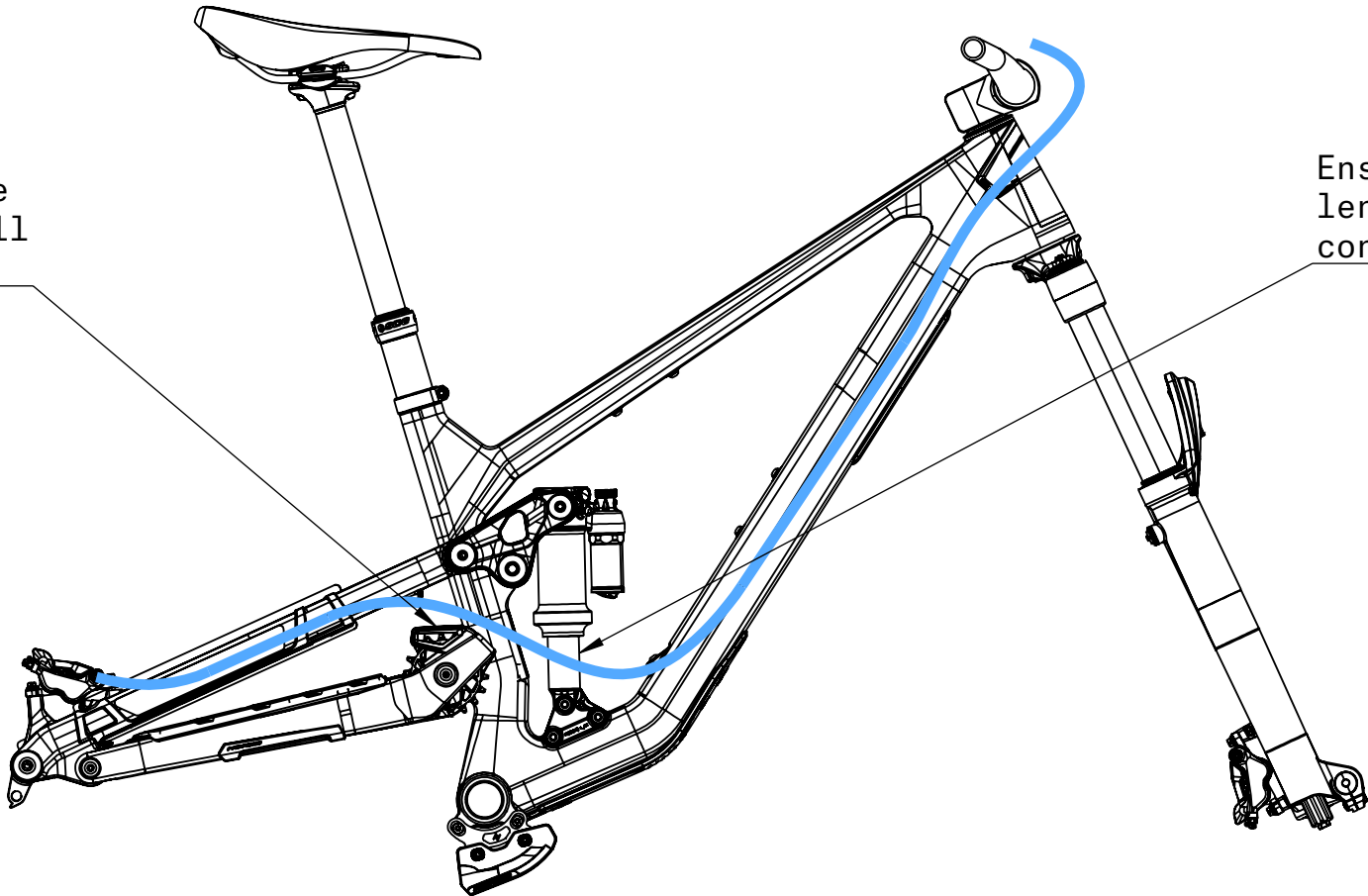
Route brake and shift housing as shown.
