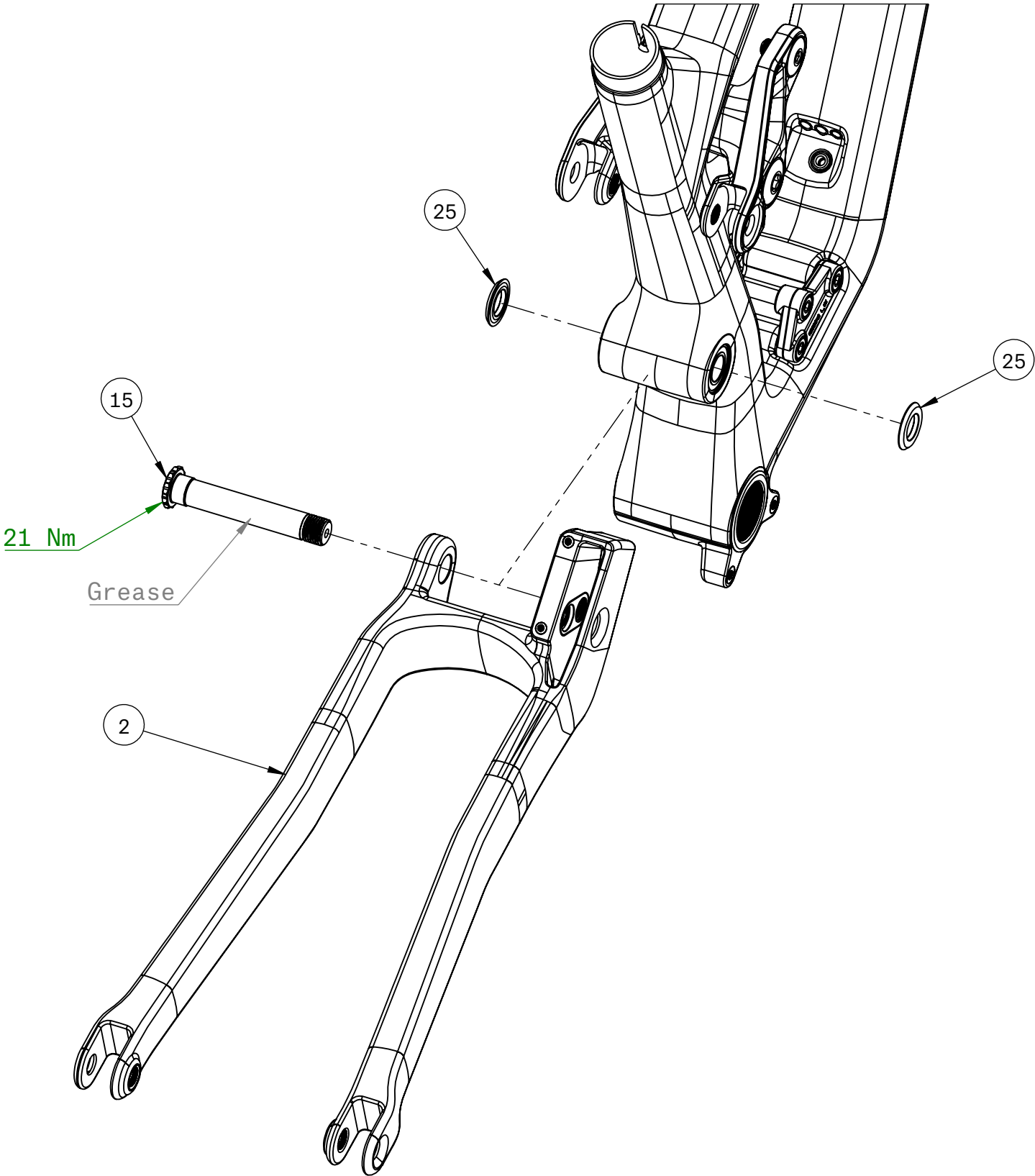
Front Triangle to Chain Stay
