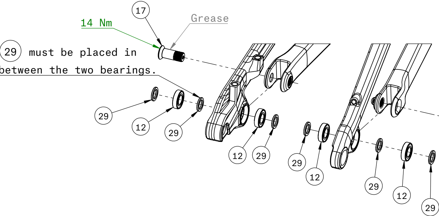
Chain Stay to Seat Stays
