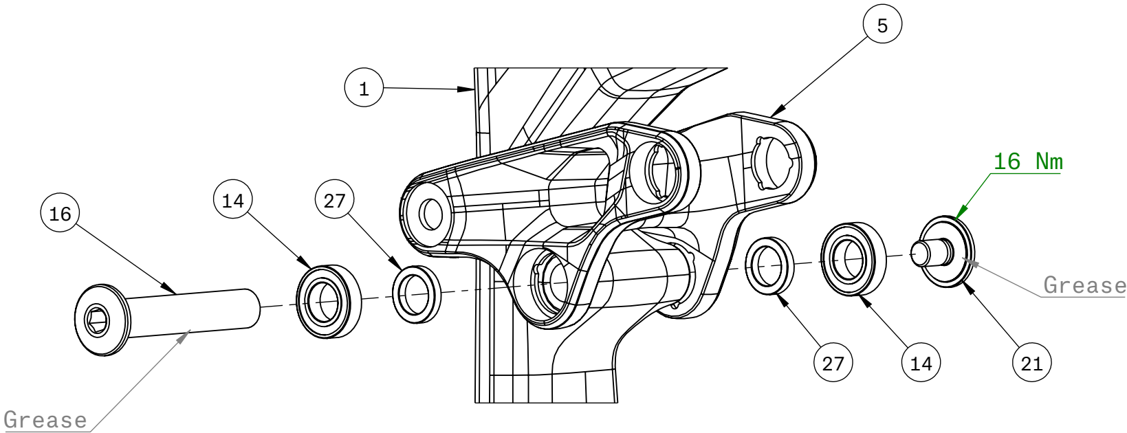
Linkarm to Front Triangle
