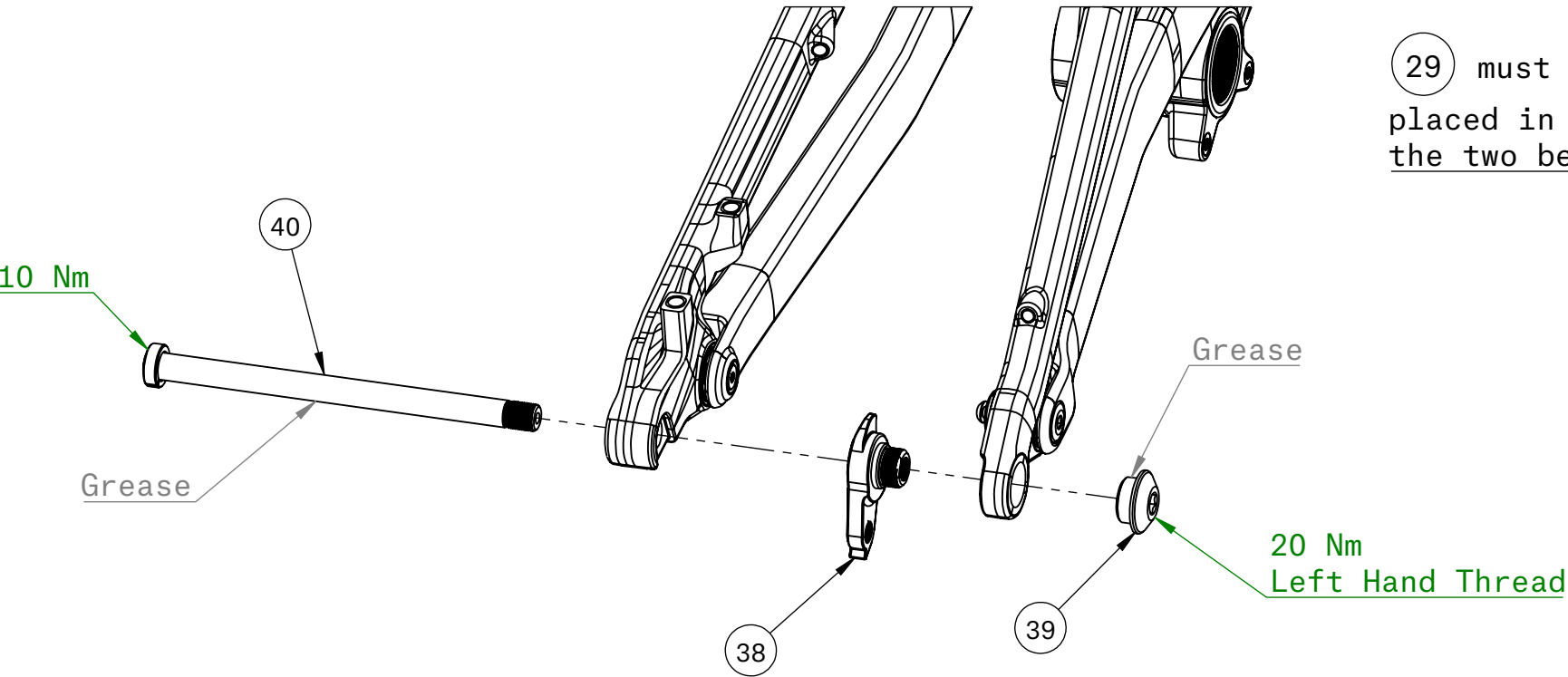
Axle and Hanger
