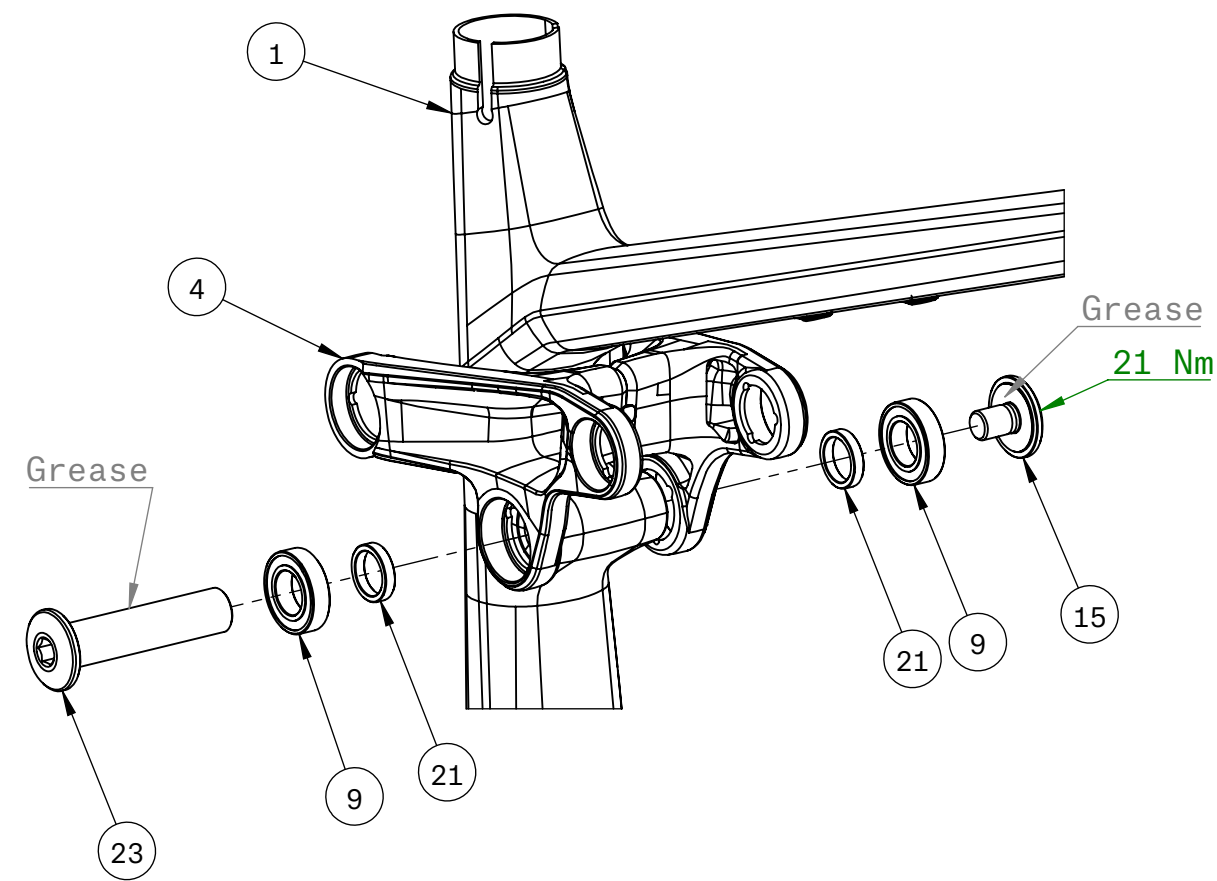
FRONT TRIANGLE TO LINKARM
