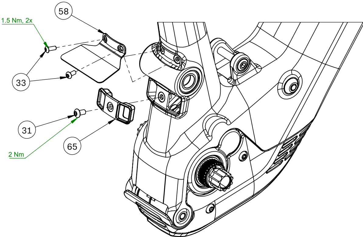
CABLE FUNNEL AND ROCK CRUSH GUARD
