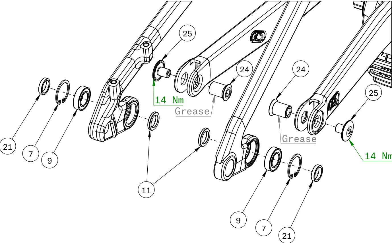
SEATSTAY TO CHAINSTAY
