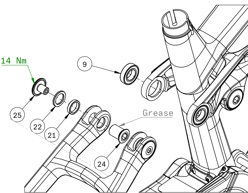
SEATSTAY TO LINKARM
