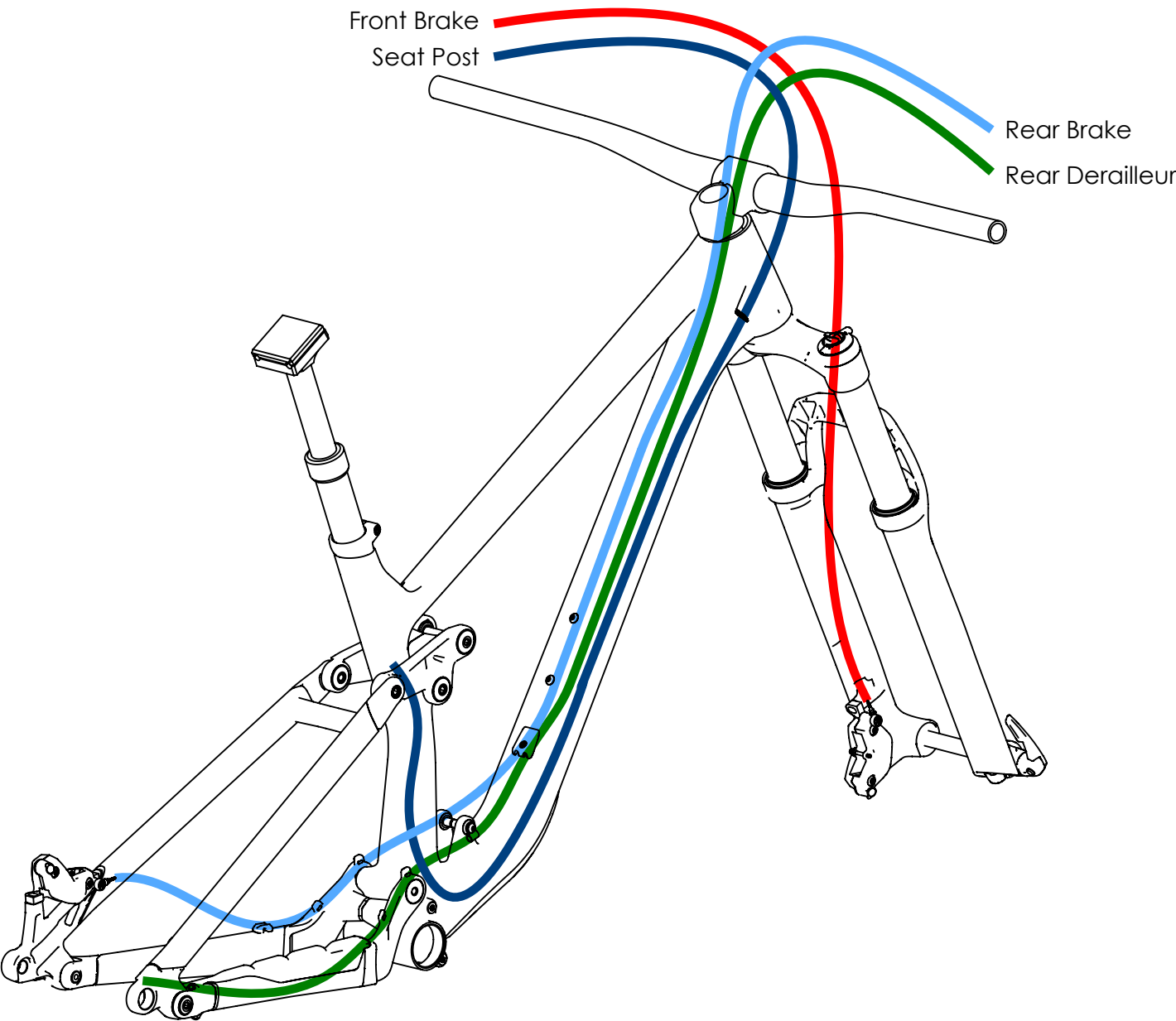
STANDARD LAYOUT ISOMETRIC VIEW
