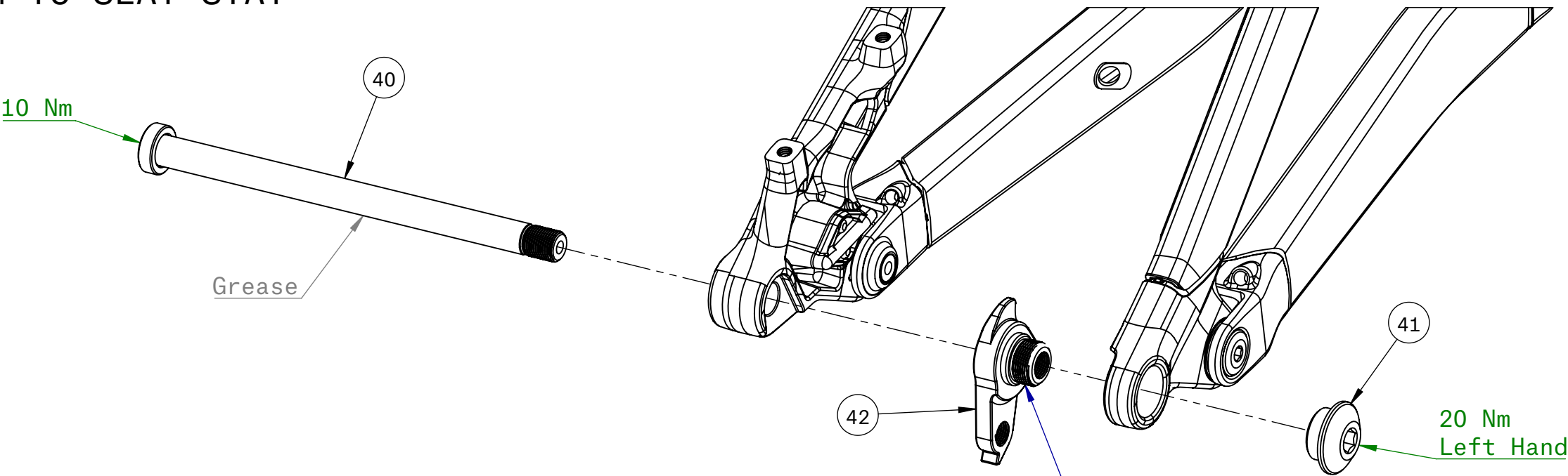
AXLE AND HANGER
