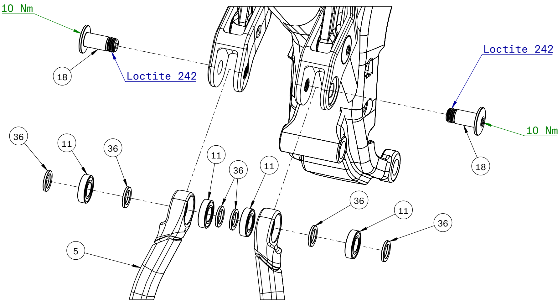
LINKARM TO SEAT STAY
