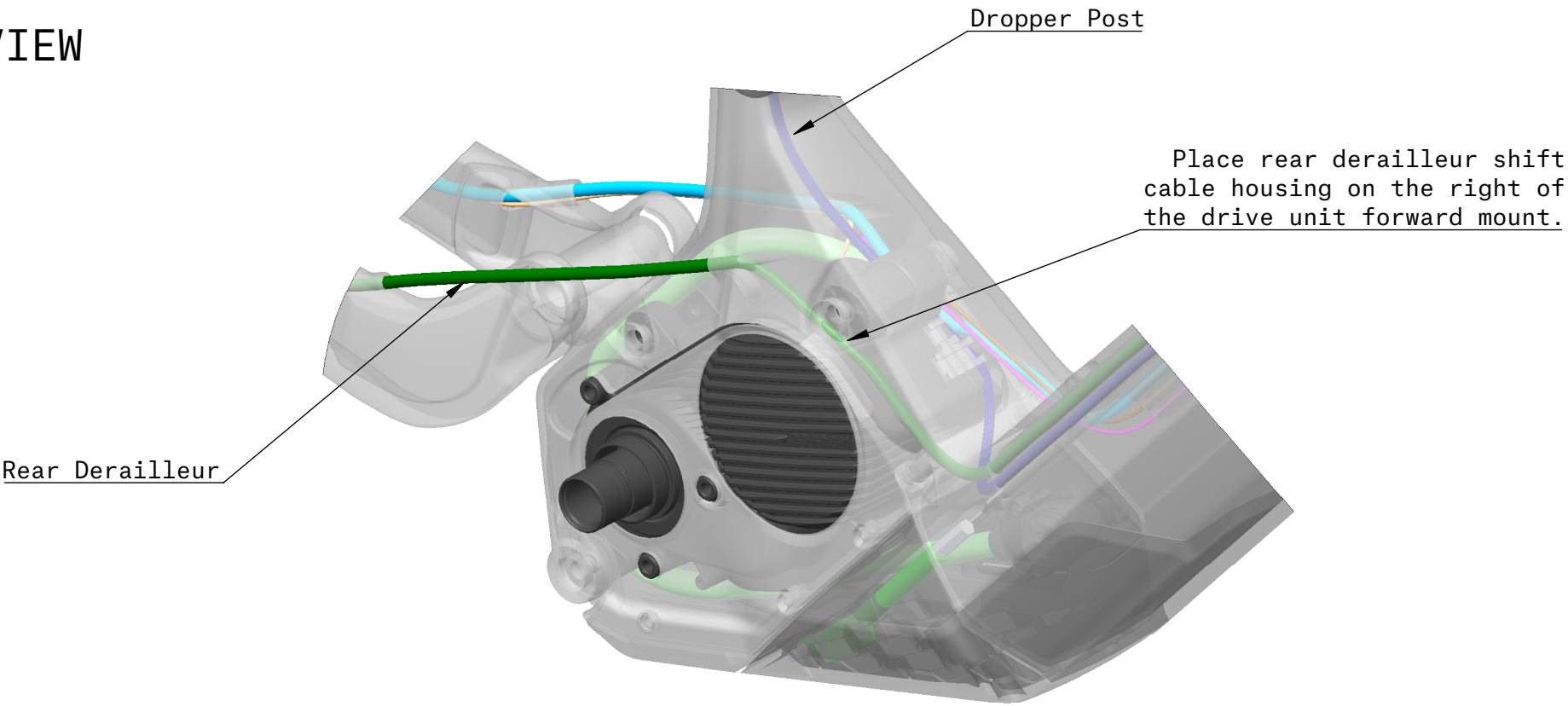
DRIVE SIDE VIEW
