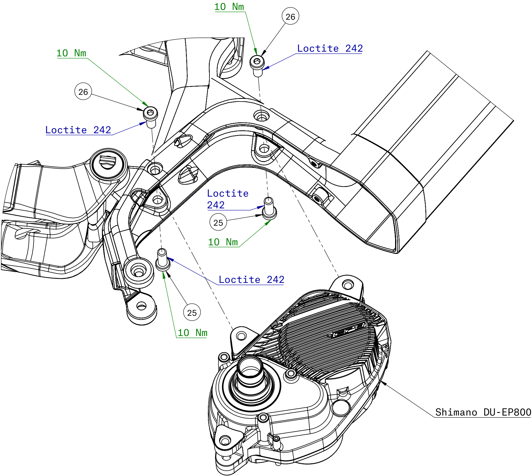
DRIVE UNIT DRIVE SIDE VIEW
