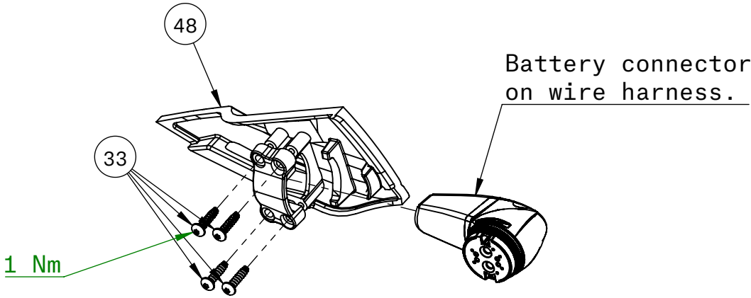
CHARGE PORT DOOR ASSEMBLY
