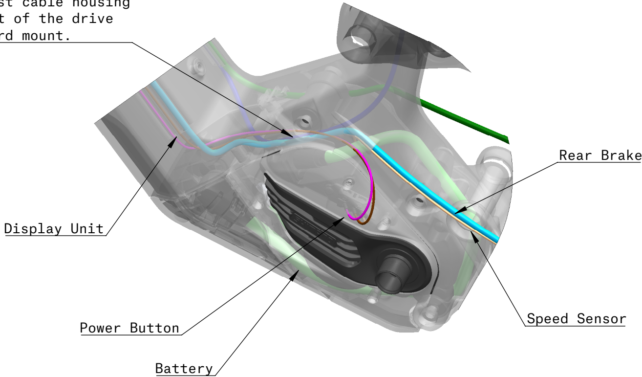
NON-DRIVE SIDE VIEW
