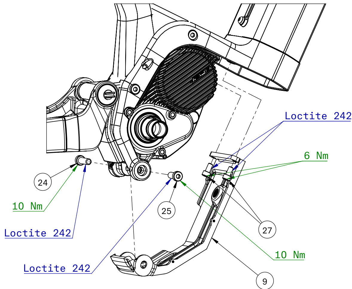
SUBFRAME DRIVE SIDE VIEW
