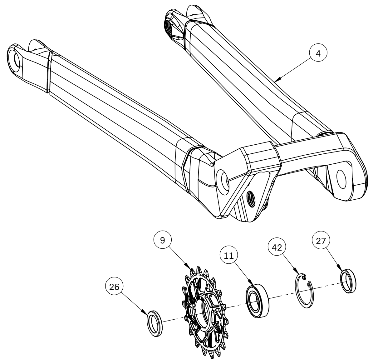
Idler Hardware Arrangement
