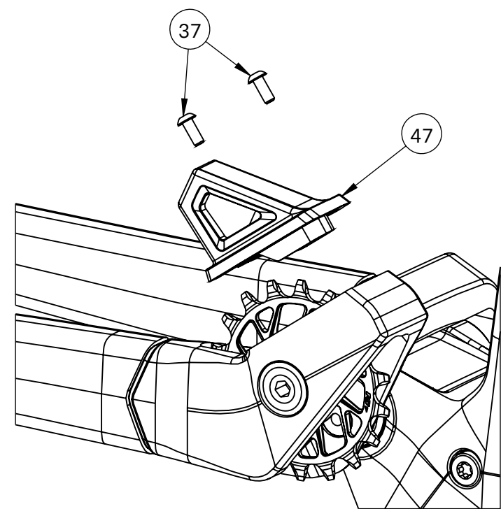
Idler Chain Guide
