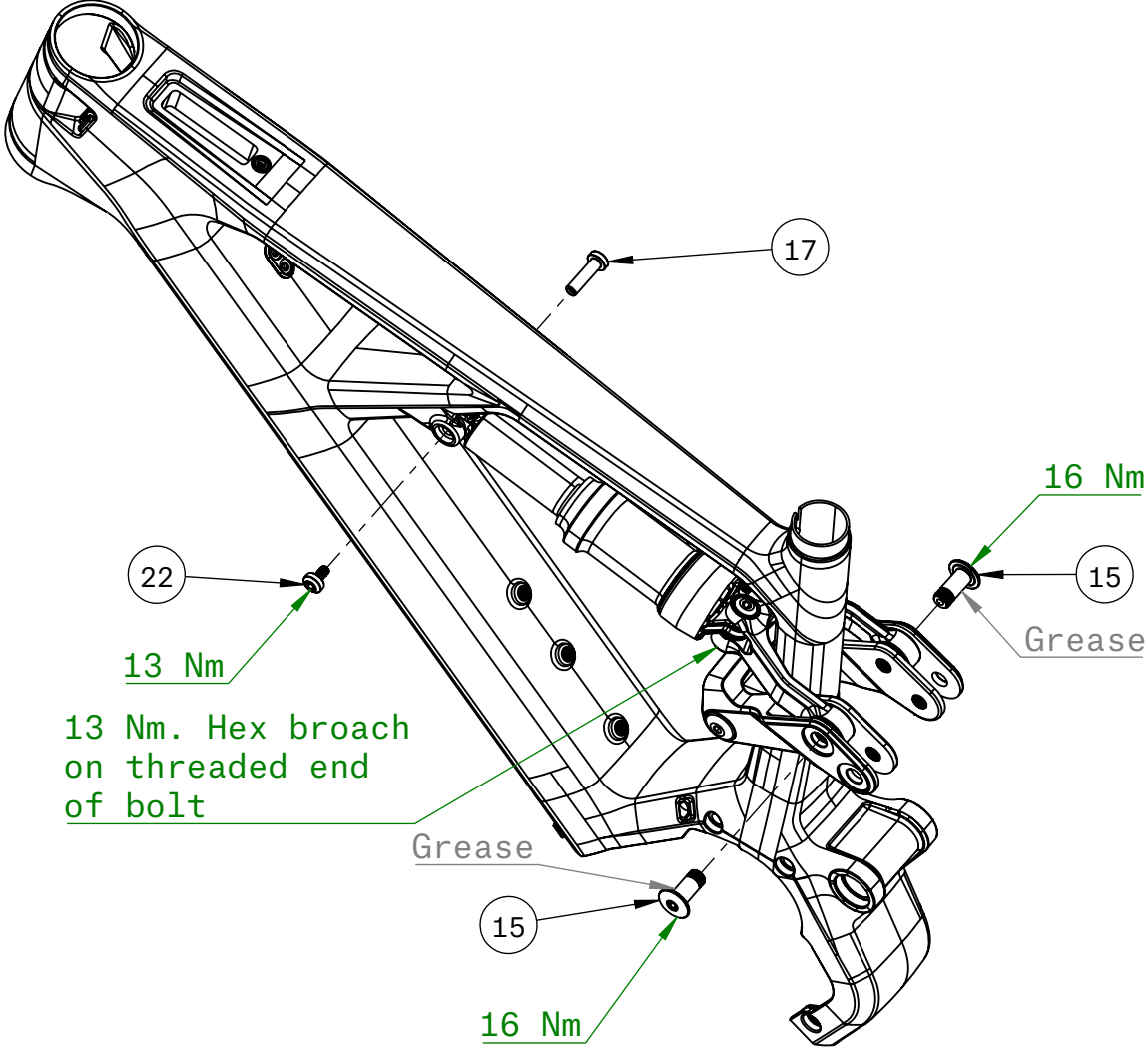
Shock Mounts
