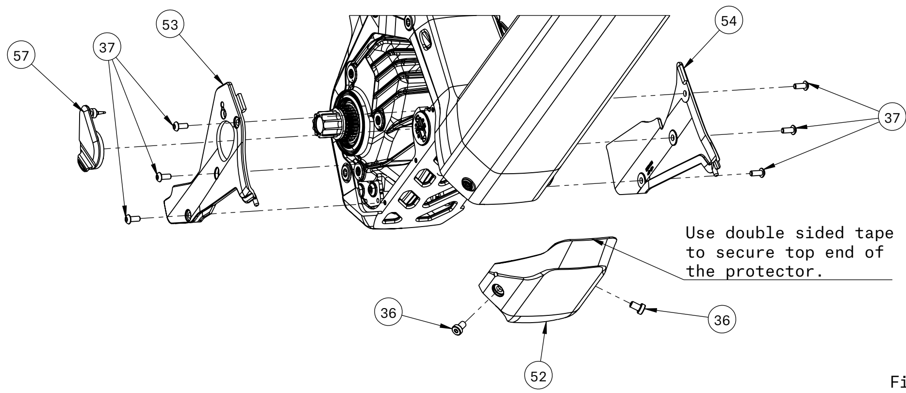
Drive Unit Covers
