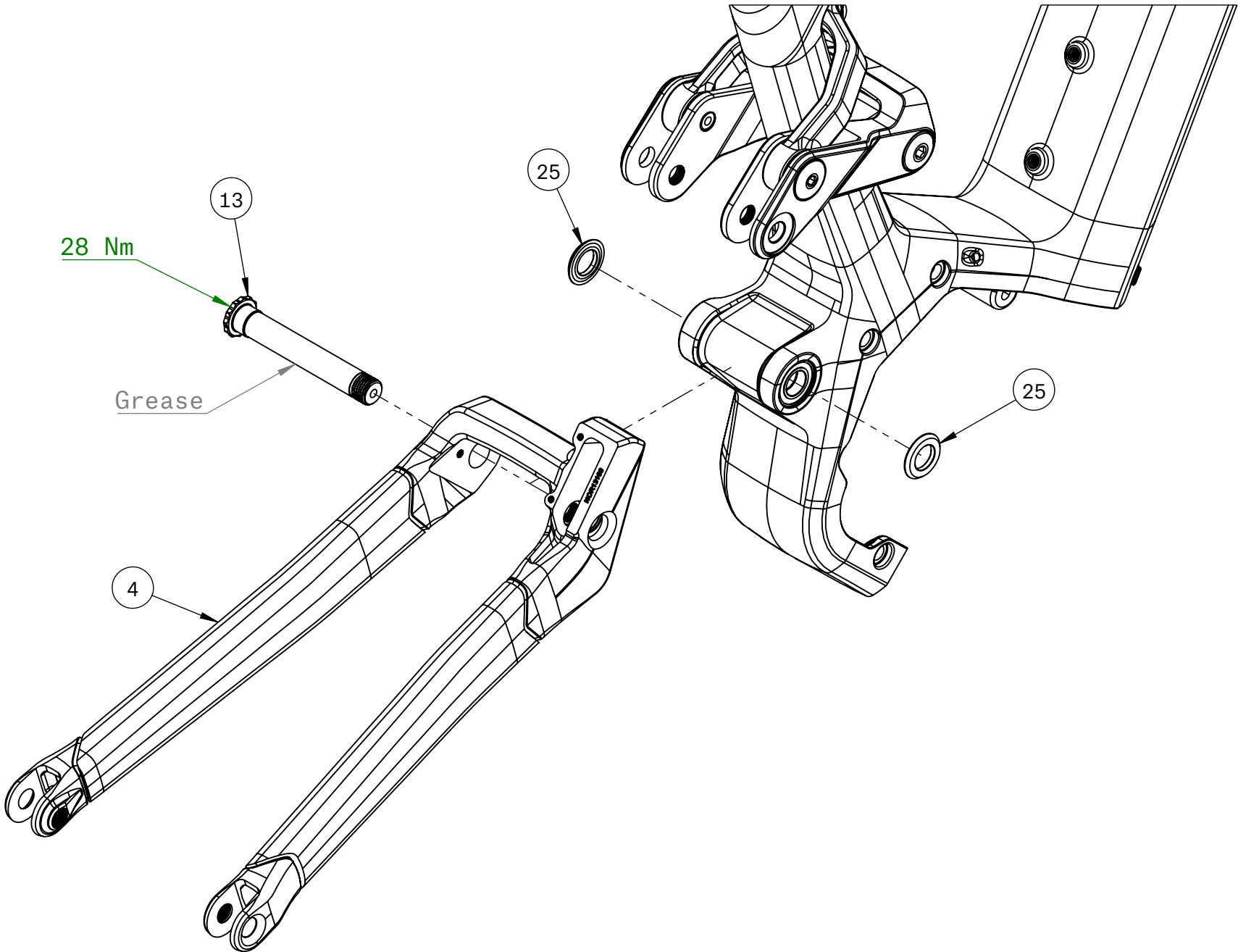
Front Triangle to Chain Stay
