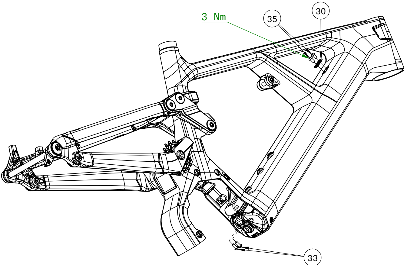
Battery Rail Installation
