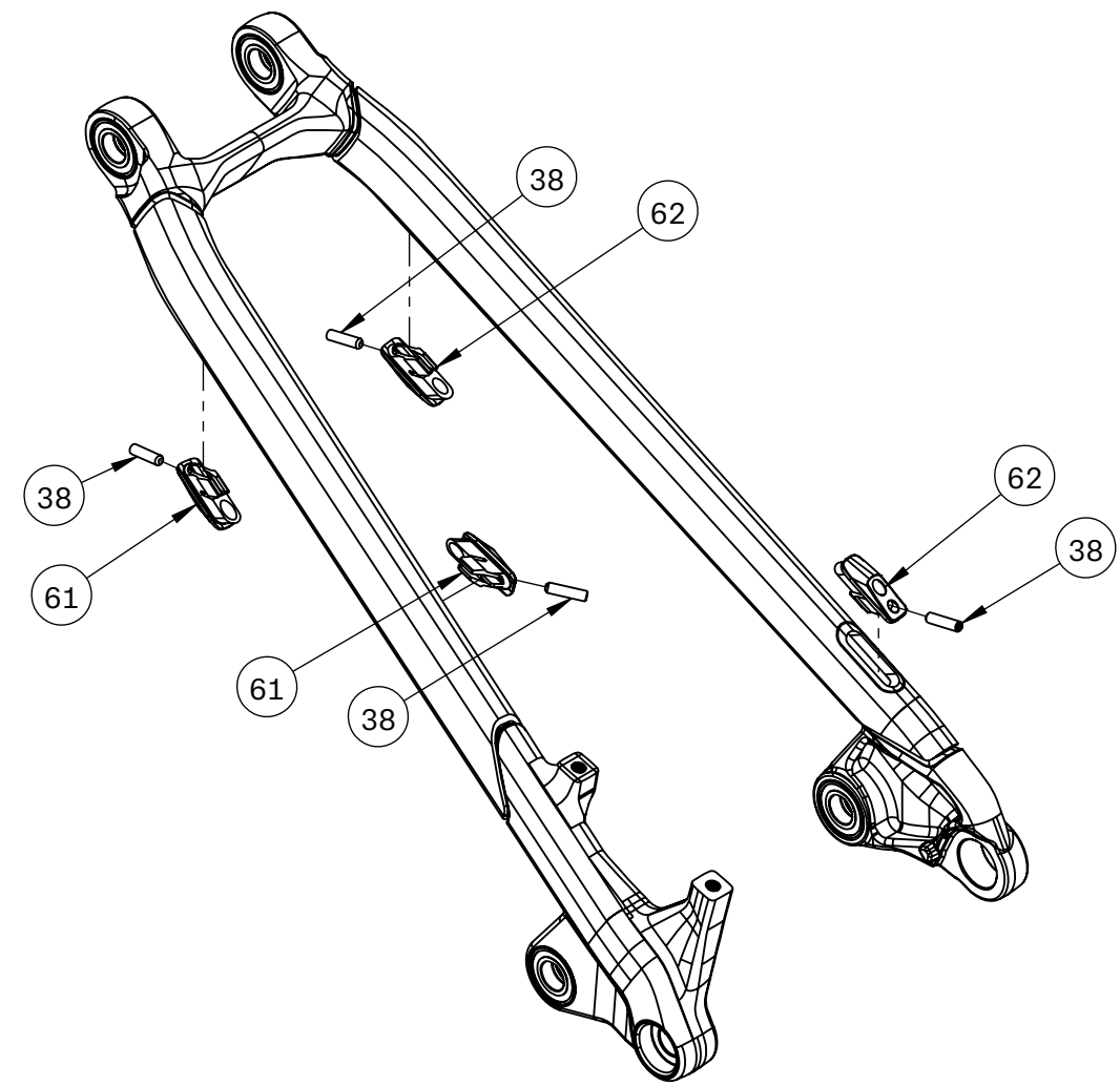
Seat Stay Cable Routing Hardware
