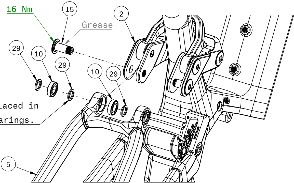
Seat Stay to Linkarm Mirrored Arrangement on Drive Side
