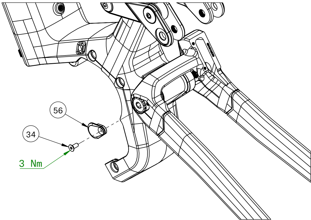
Main Pivot Shaft Retainer
