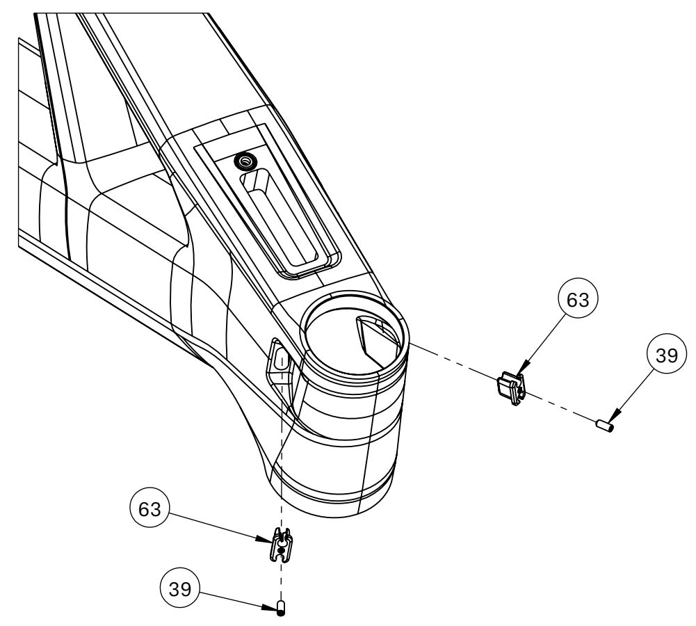
Head Tube Cable Routing Hardware
