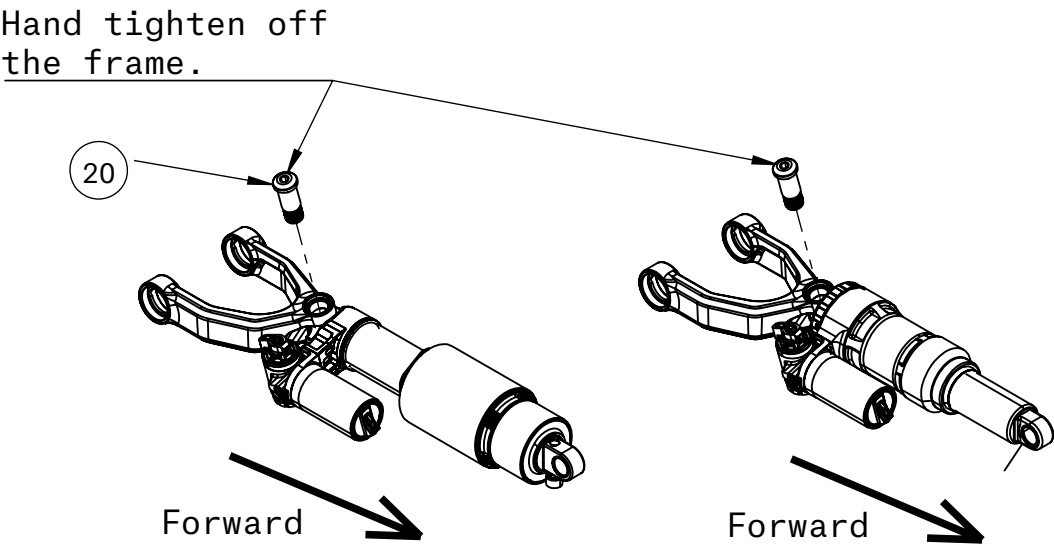
Shock Mounts
