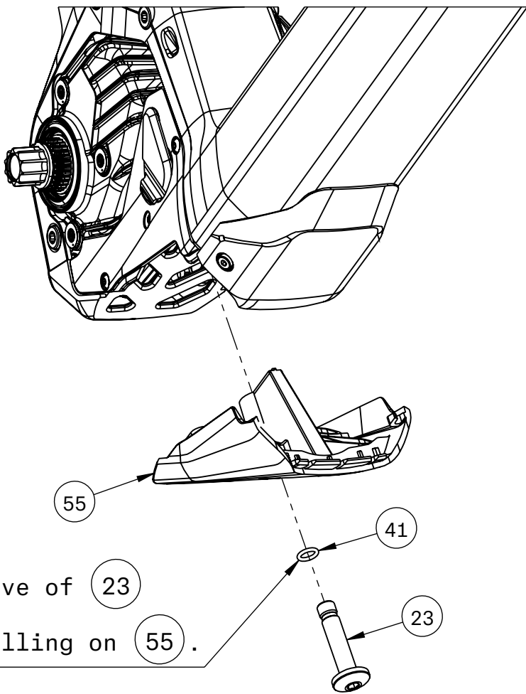
Lower Cover
