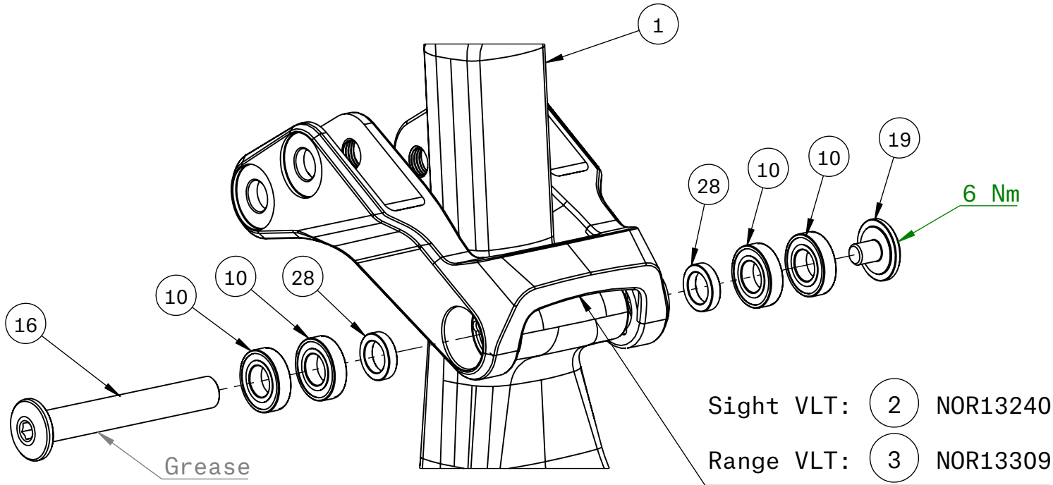
Linkarm to Front Triangle
