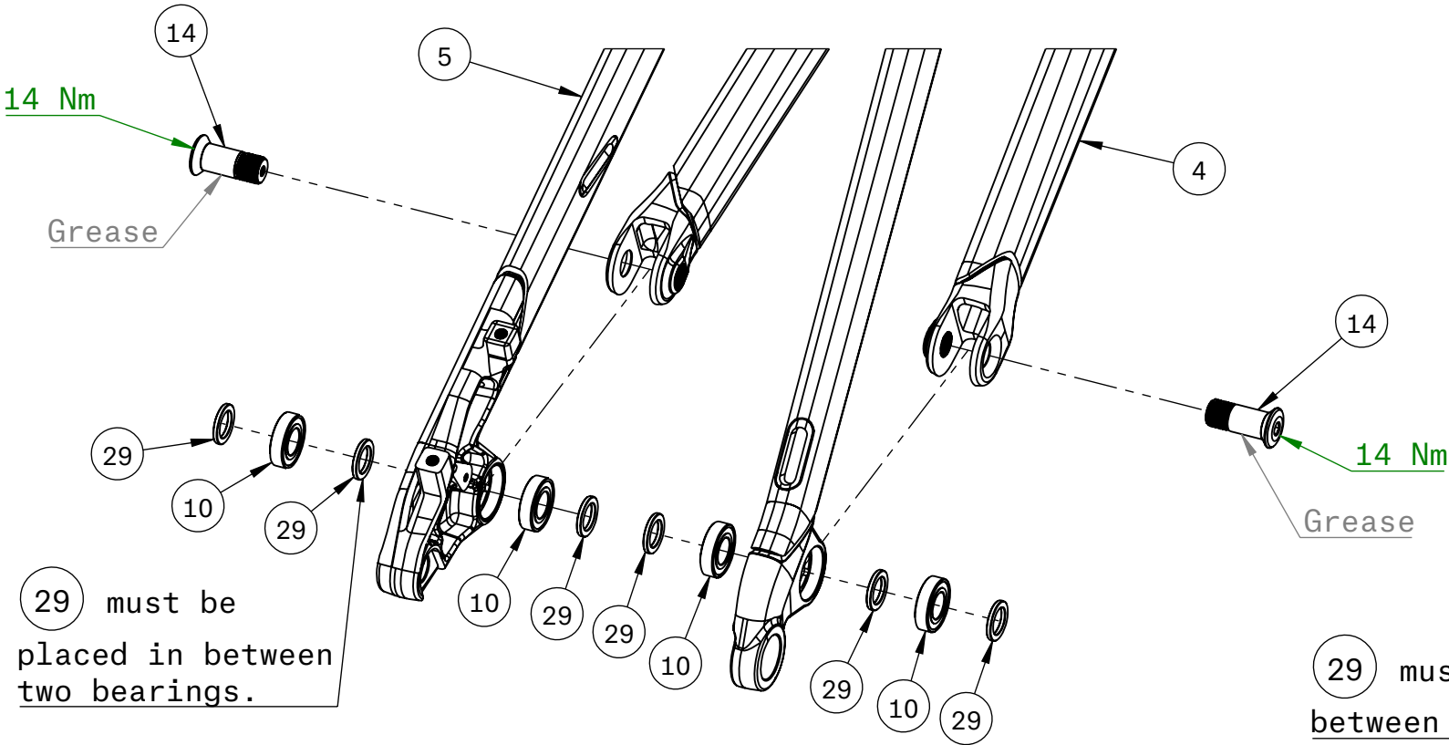
Seat Stay to Chain Stay
