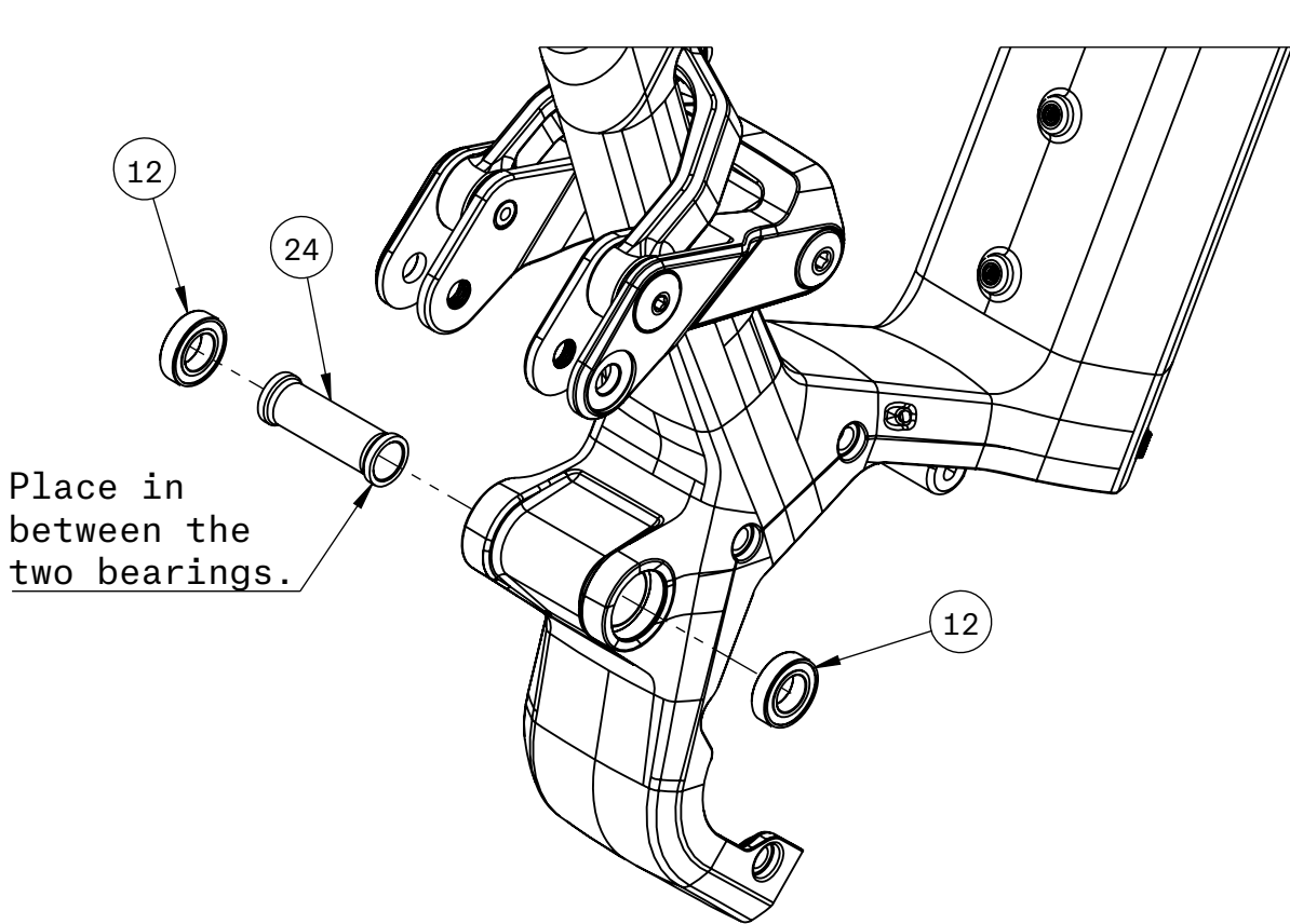
Front Triangle Bearings
