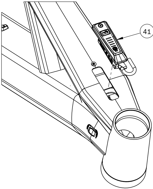
Tuptube Controller
