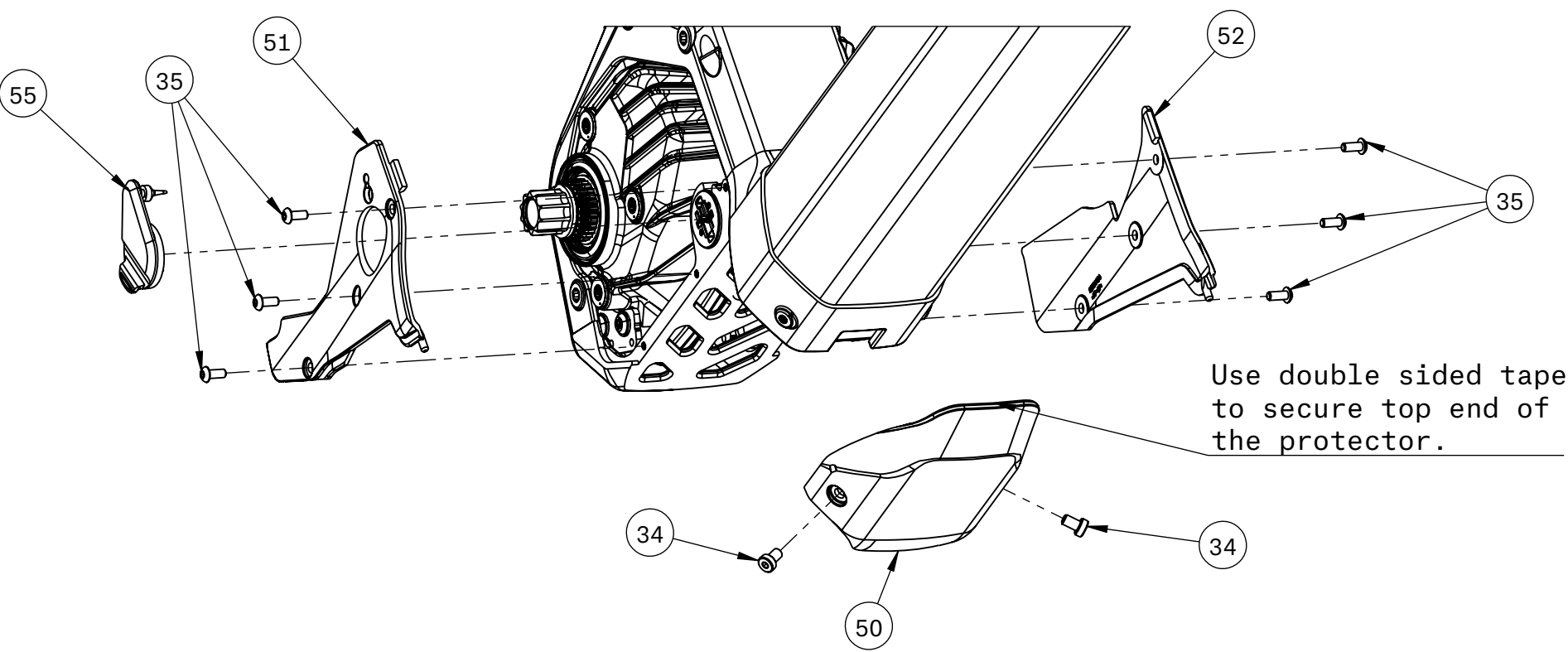
Drive Unit Covers
