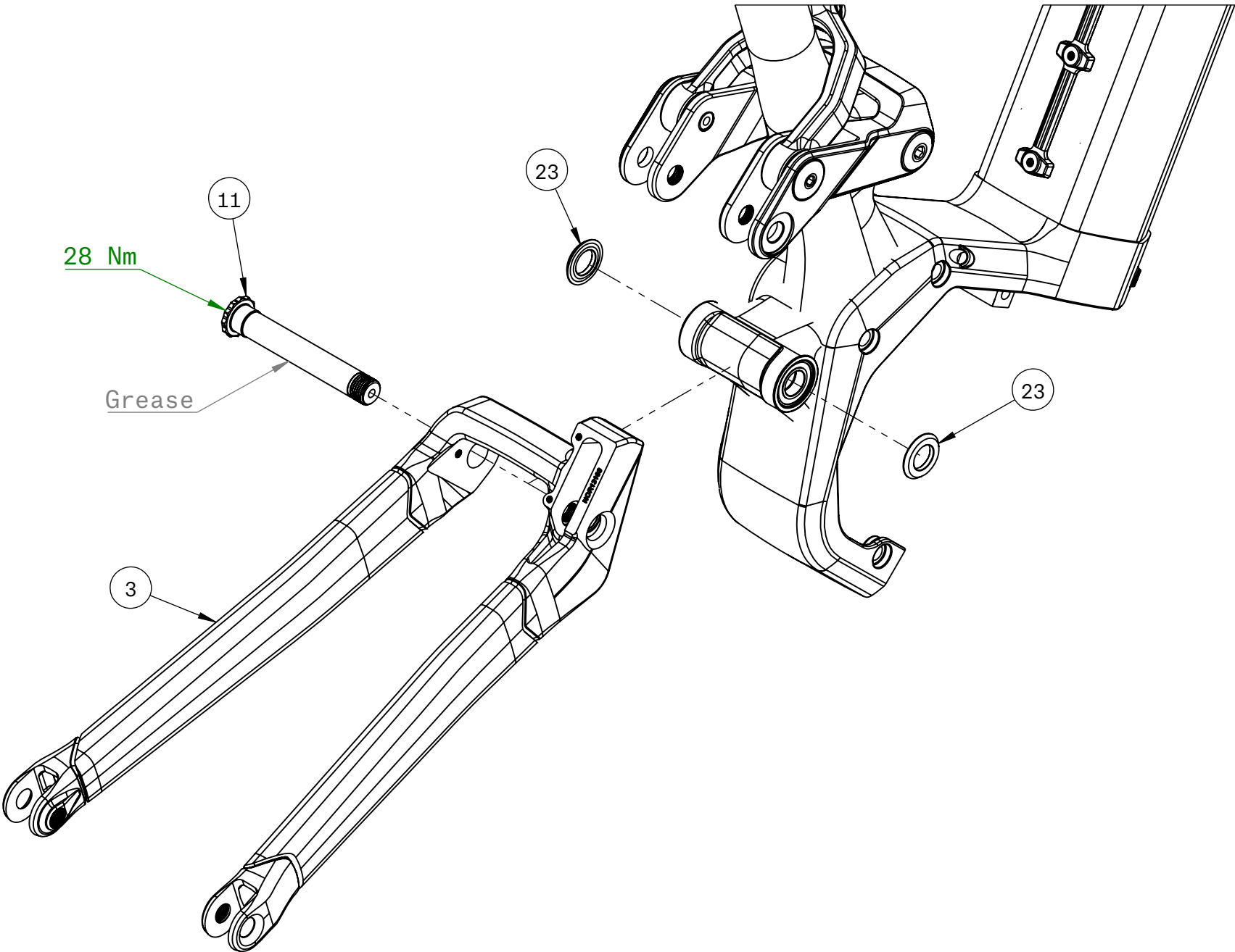
Front Triangle to Chain Stay
