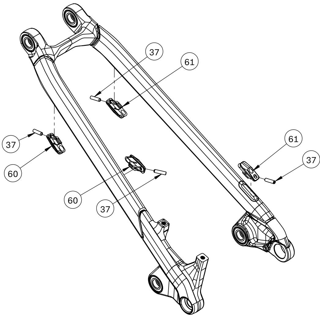
Seat Stay Cable Routing Hardware
