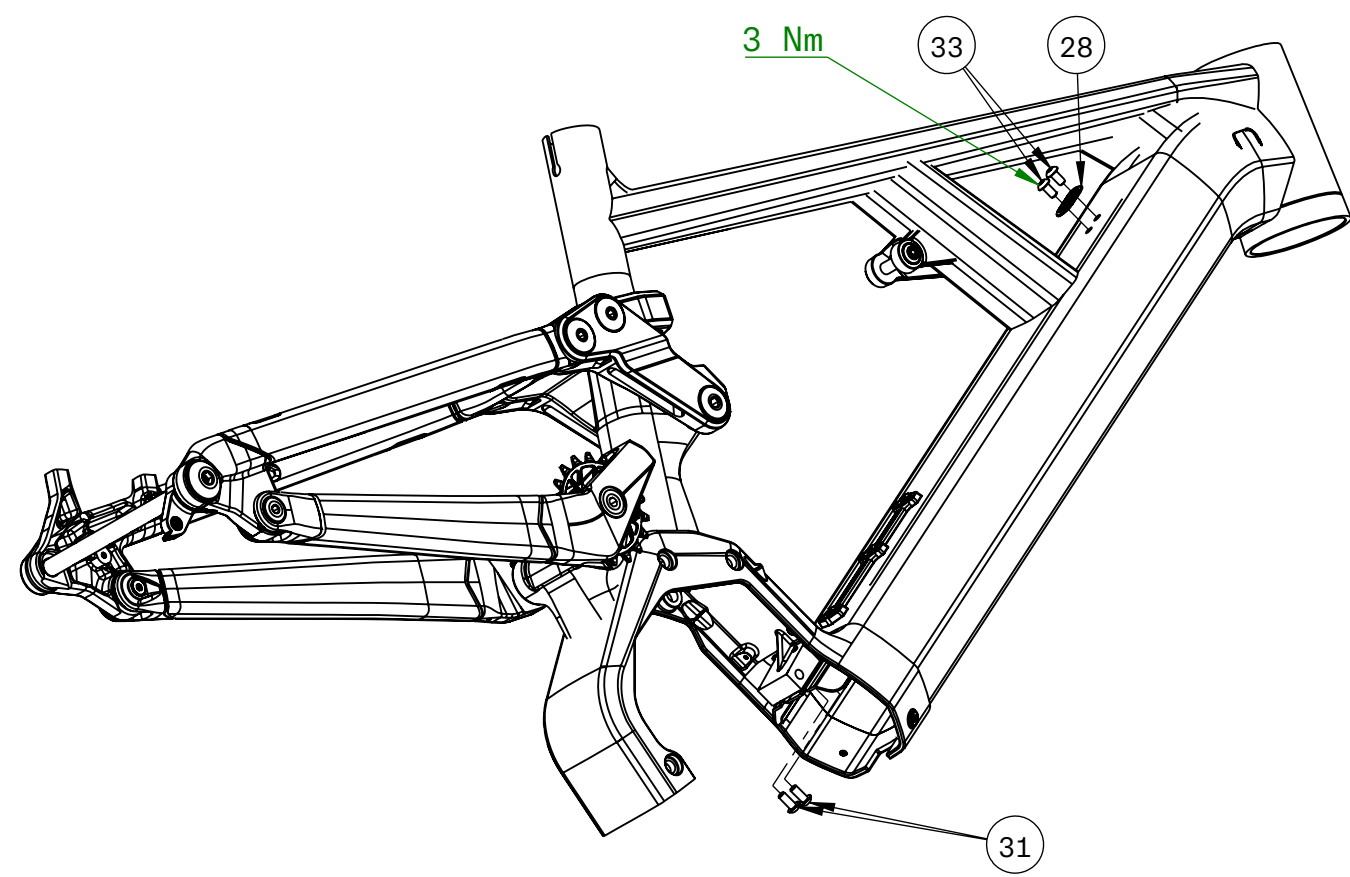
Battery Rail Installation
