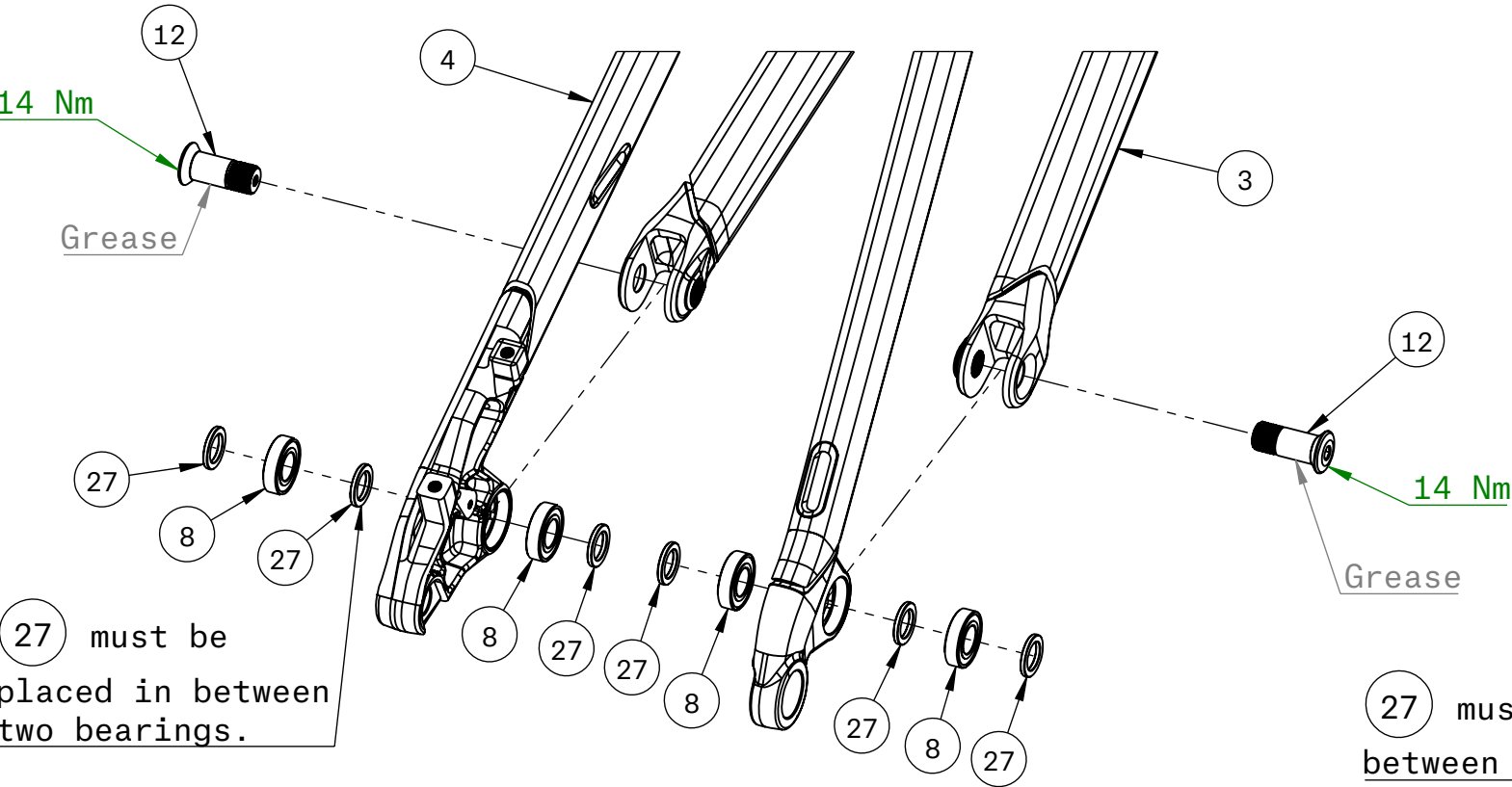
Seat Stay to Chain Stay
