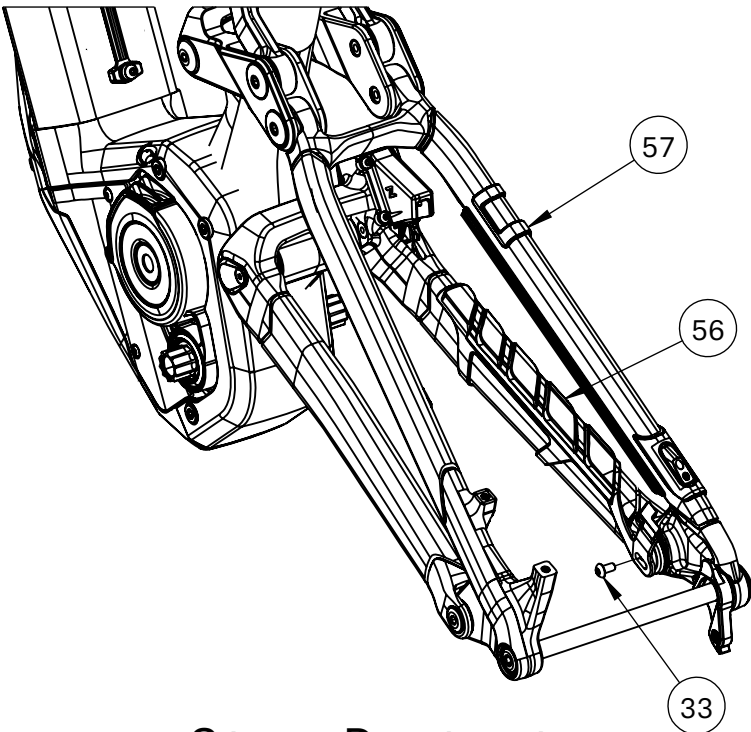
Stay Protectors
