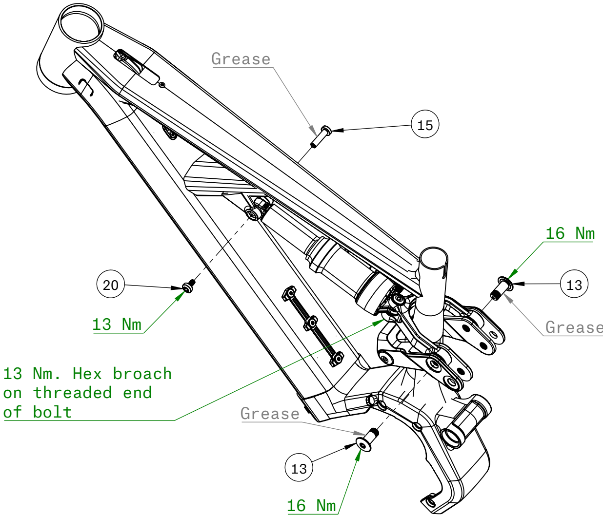
Shock Mounts
