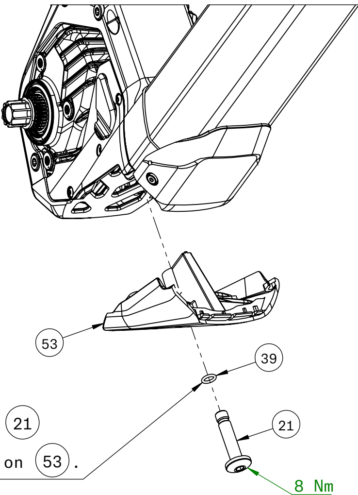
Lower Cover
