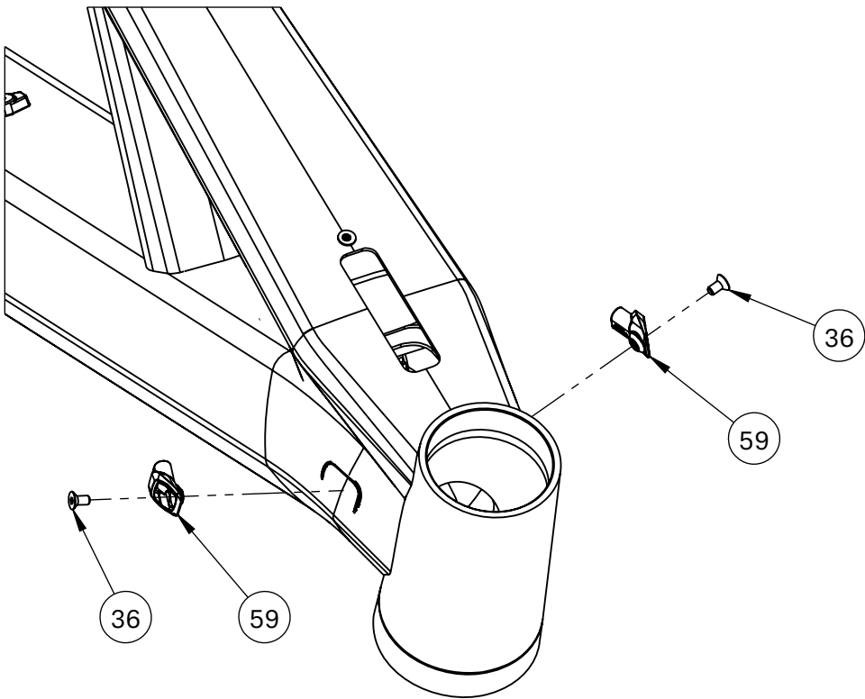
Head Tube Cable Routing Hardware
