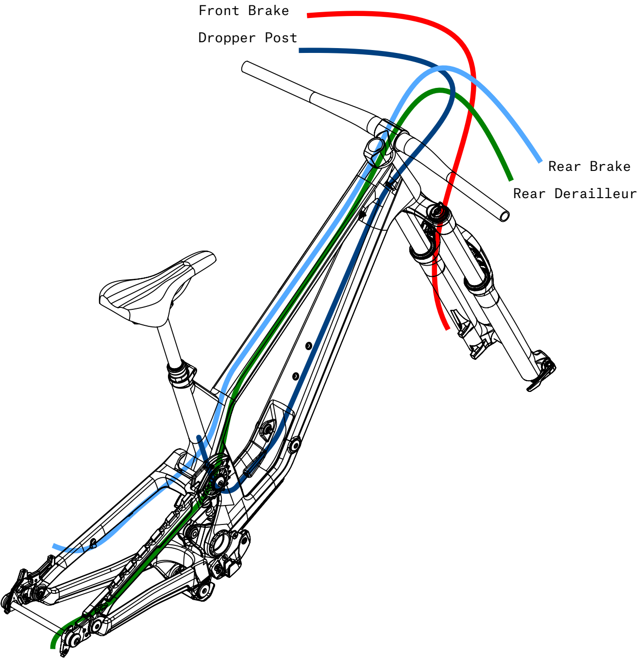
STANDARD LAYOUT ISOMETRIC VIEW
