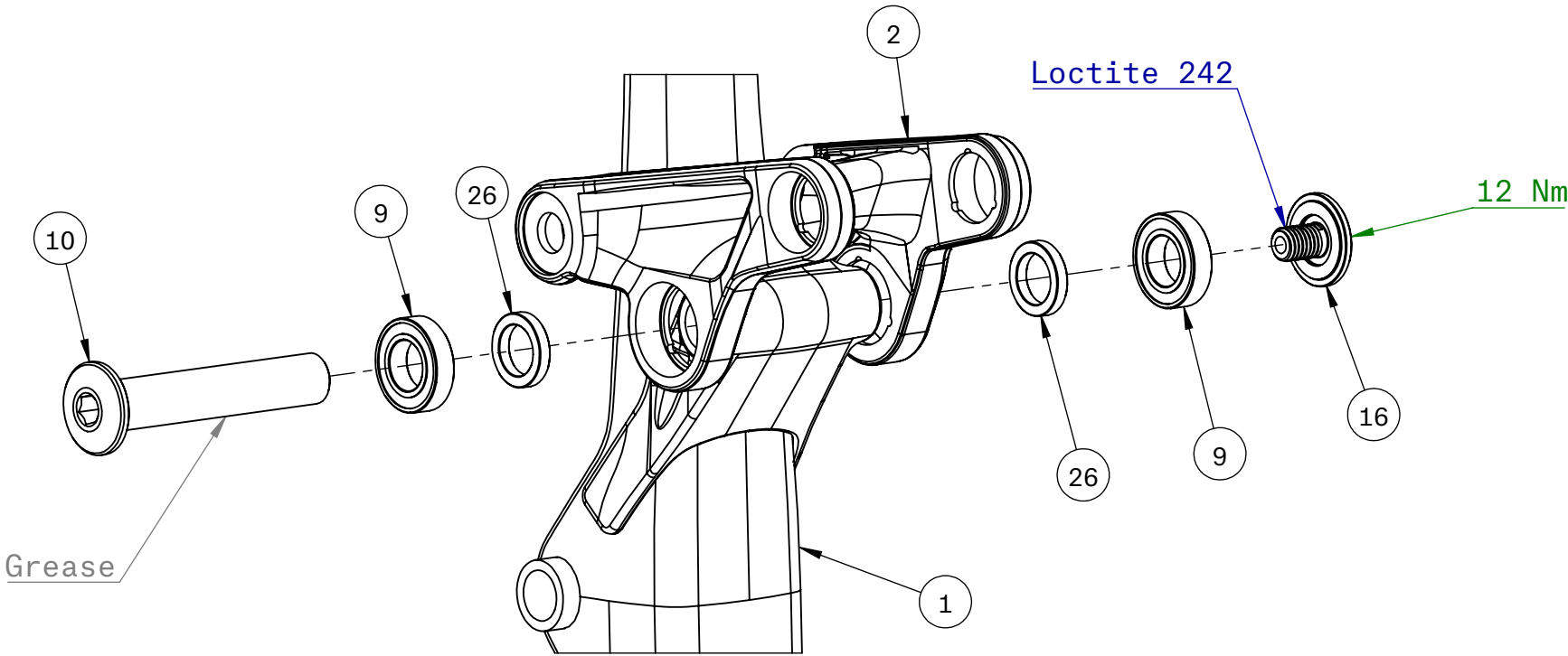
FRONT TRIANGLE TO LINKARM PIVOT
