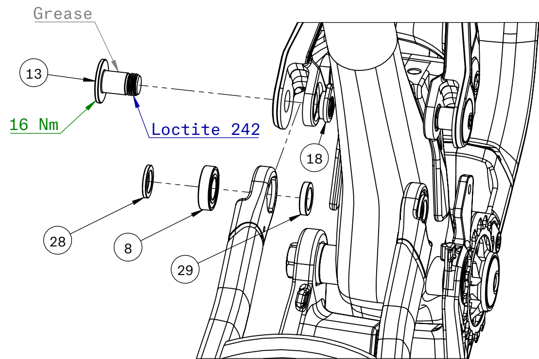
LINKARM TO SEAT STAY PIVOT SAME ARRANGEMENT ON BOTH SIDES
