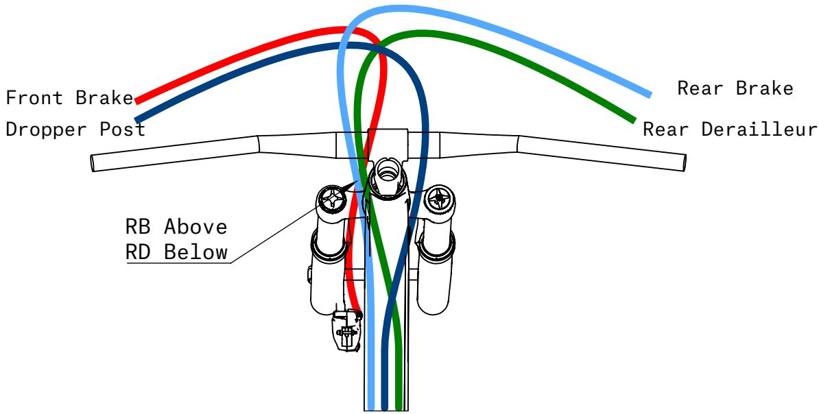
STANDARD LAYOUT
