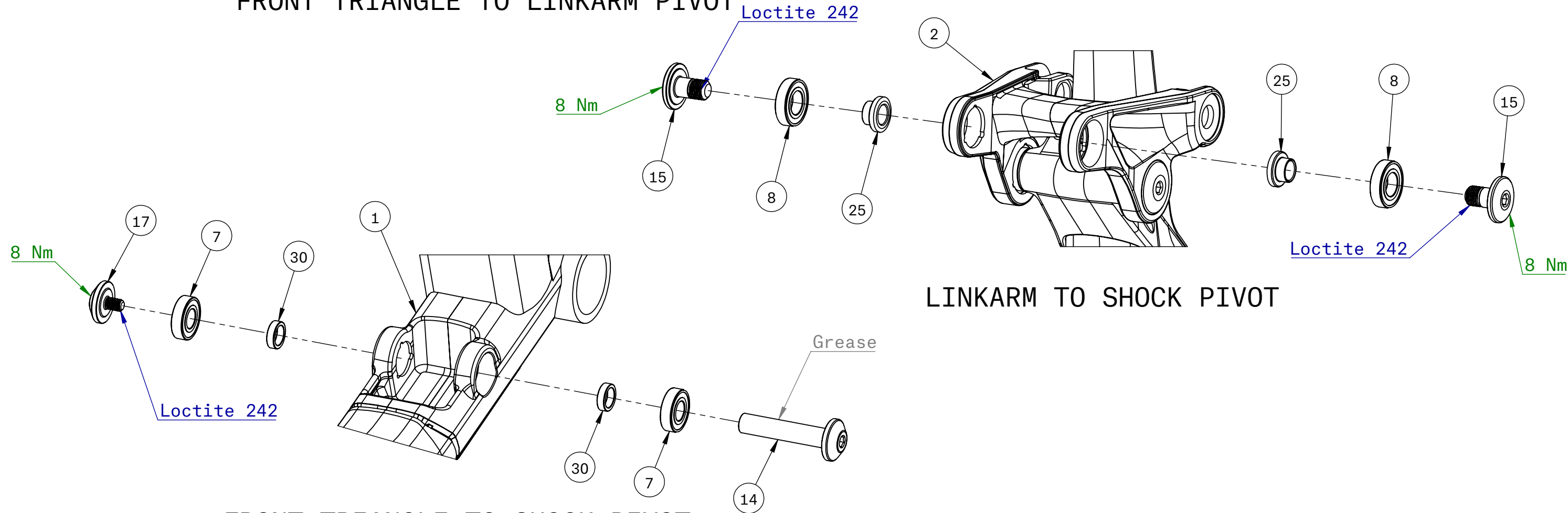
FRONT TRIANGLE TO SHOCK PIVOT
