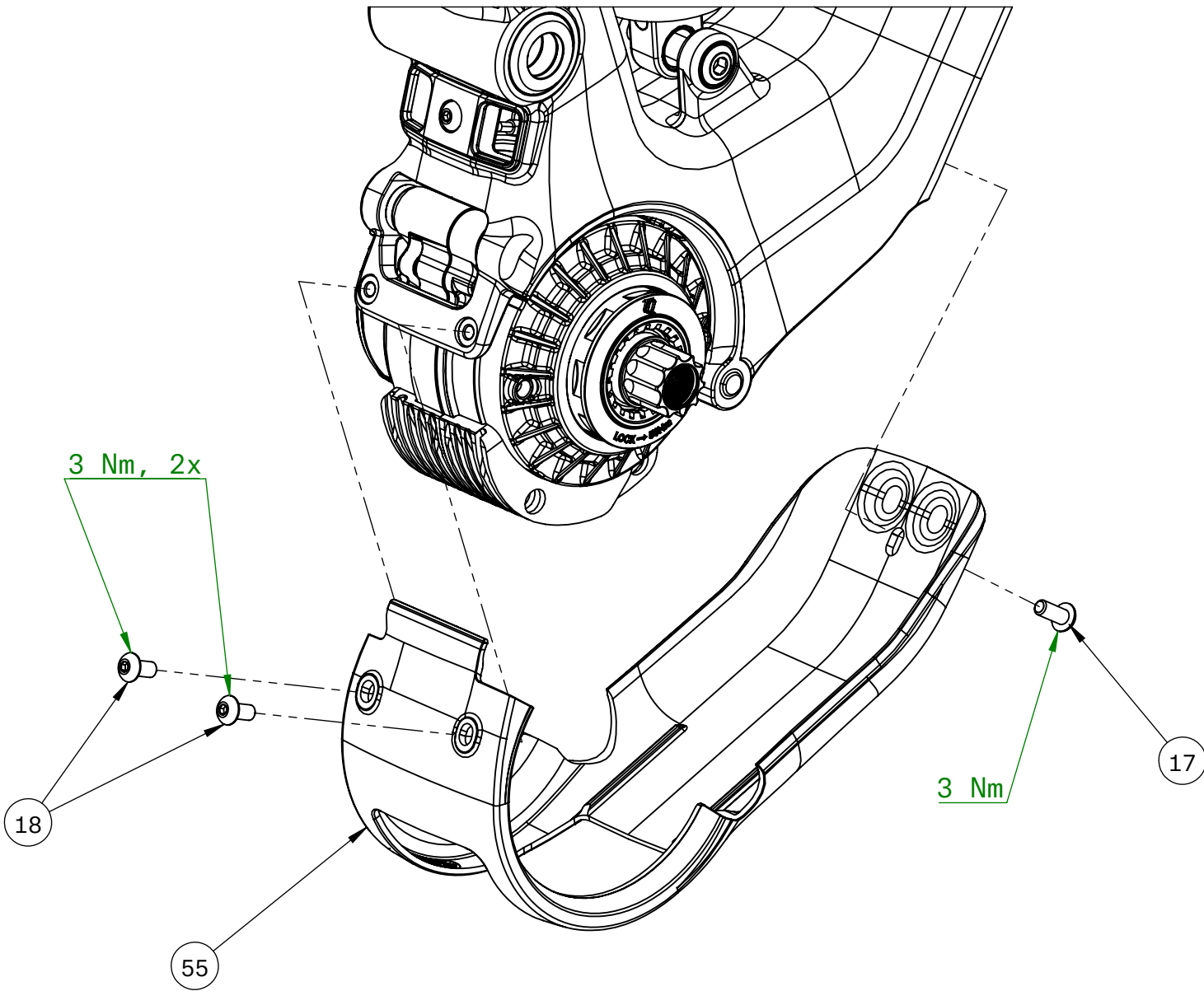
MOTOR COVER
