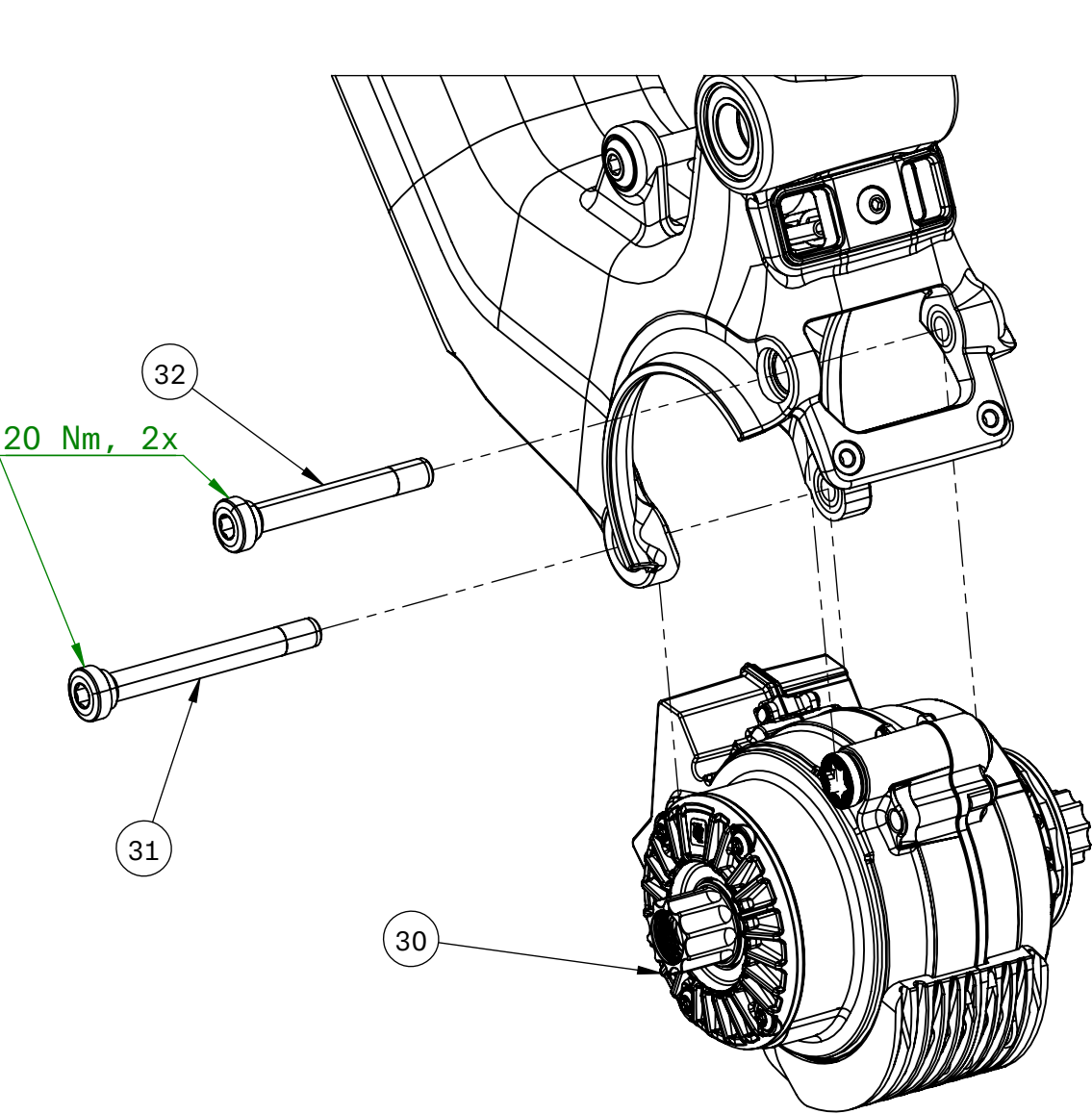
DRIVE UNIT
